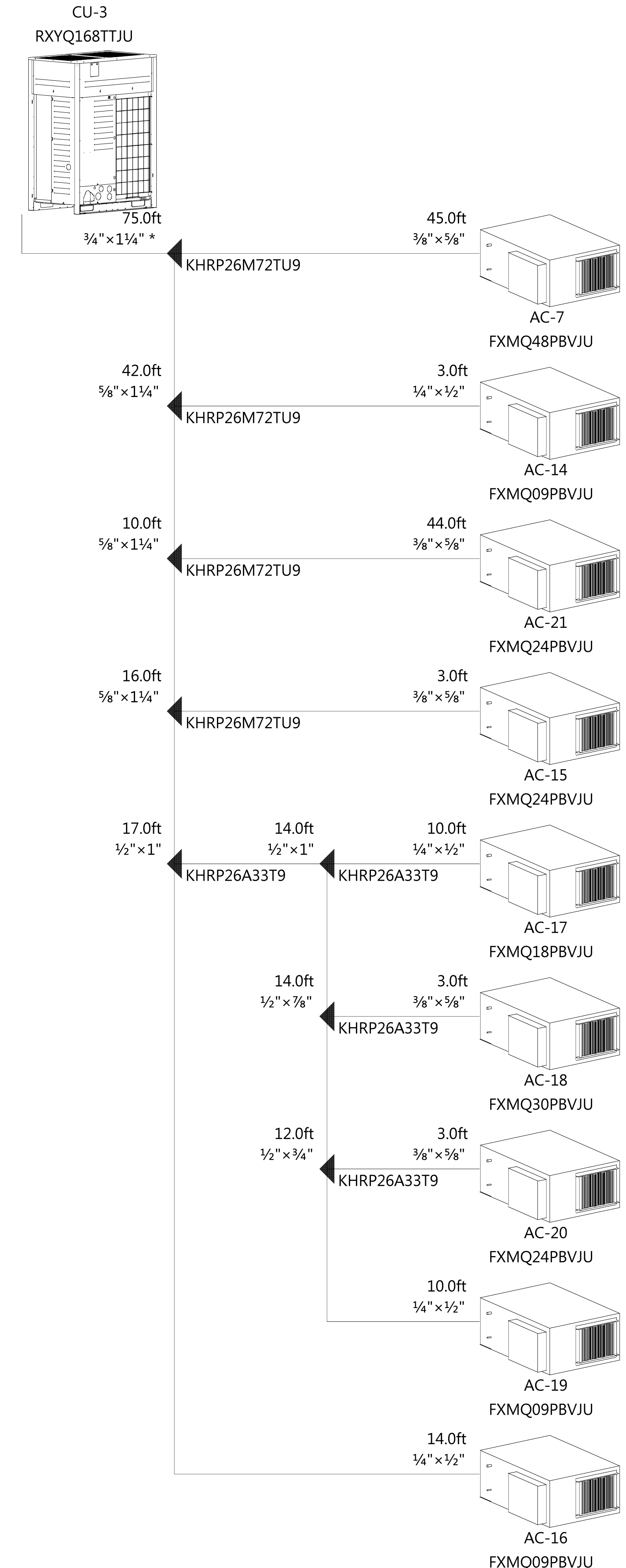
3 CU-3 PIPING DETAIL NO SCALE
