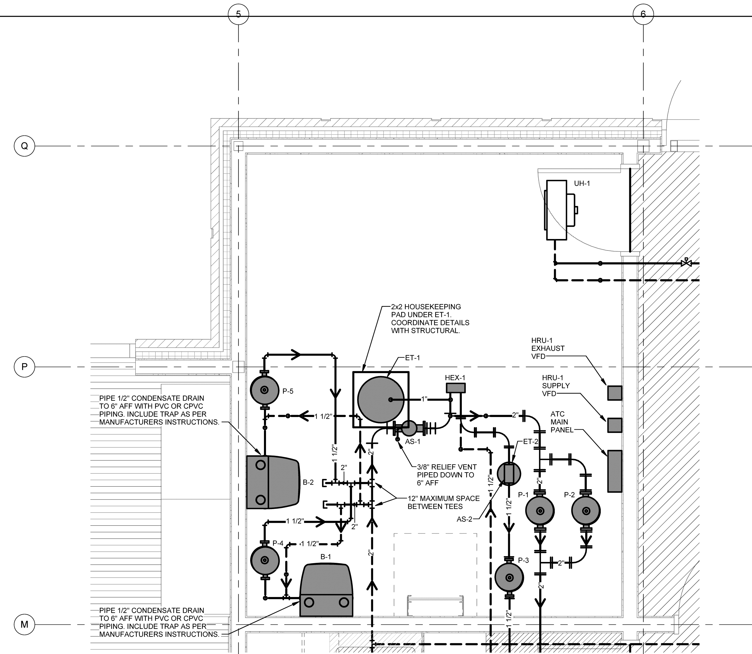
2 MECHANICAL ROOM PART PLAN NO SCALE
