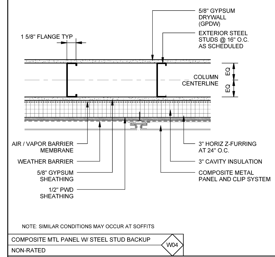
COMPOSITE MTL PANEL W/ STEEL STUD BACKUP
