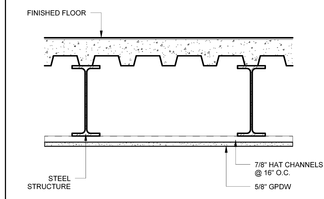
GPDW CEILING SYSTEM ON STRUCTURE
