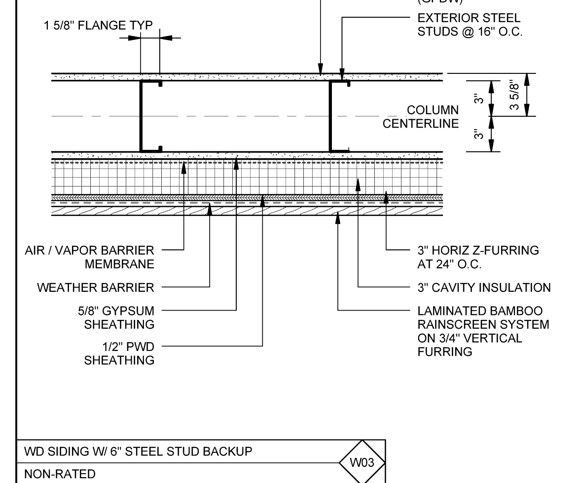
WD SIDING W/ 6" STEEL STUD BACKUP
