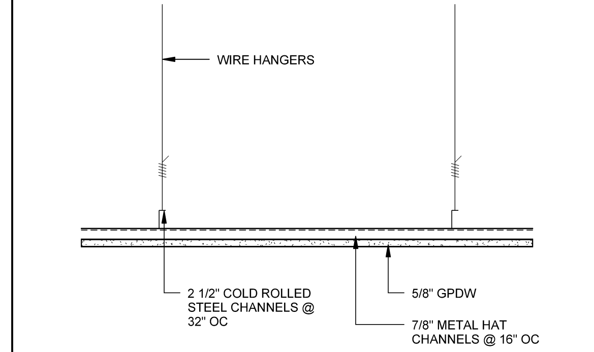
SUSPENDED GPDW CEILING SYSTEM
