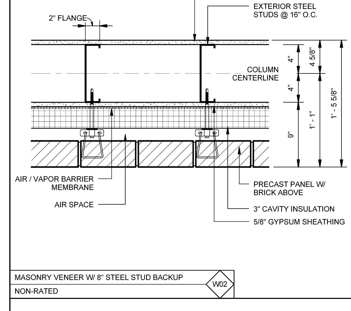
MASONRY VENEER W/ 8" STEEL STUD BACKUP
