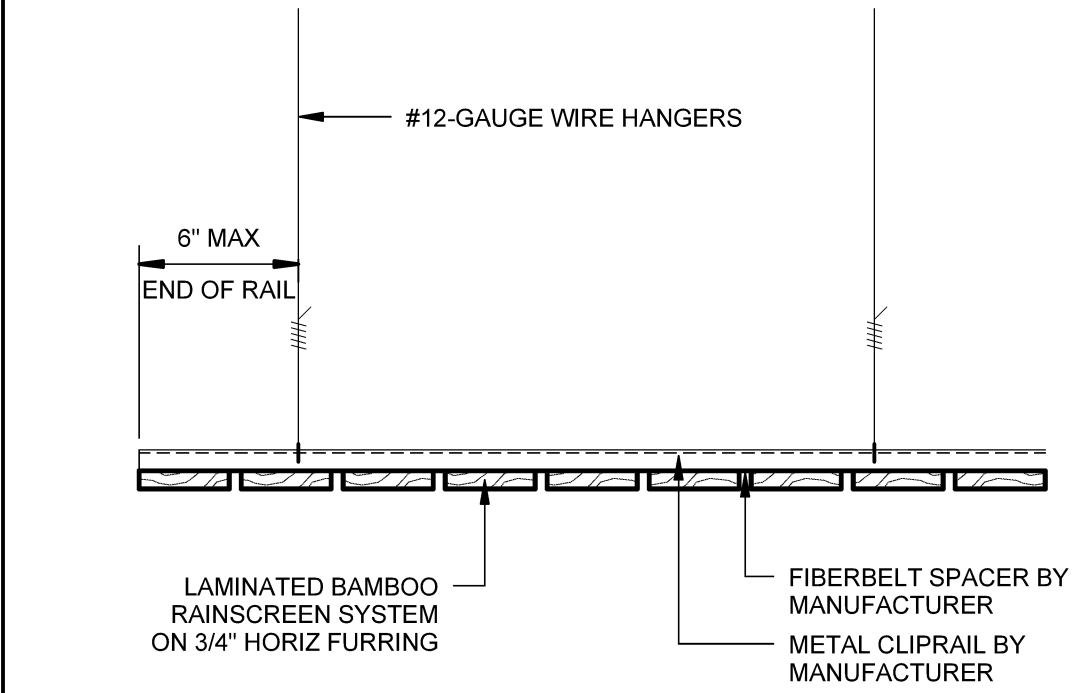
SUSPENDED WOOD CEILING SYSTEM
