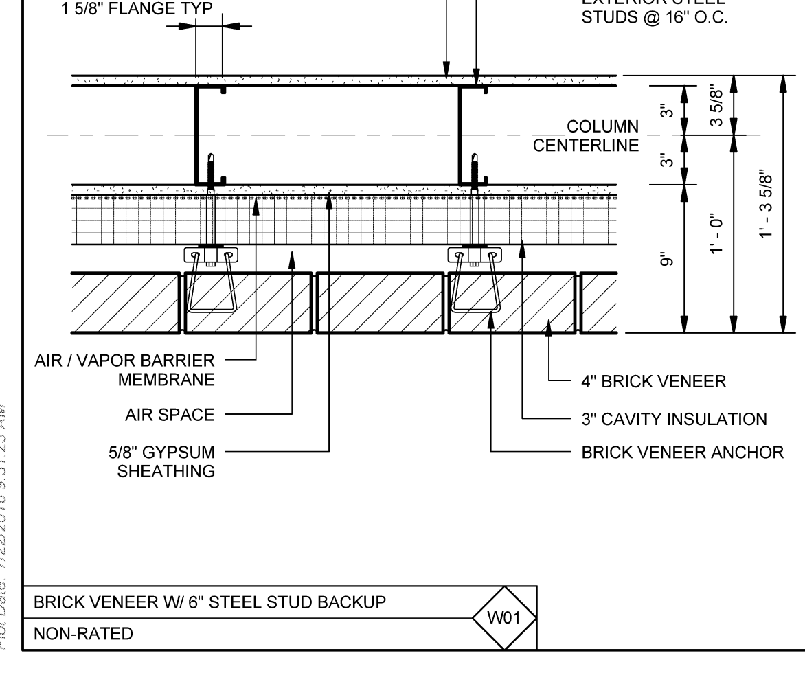
BRICK VENEER W/ 6" STEEL STUD BACKUP
