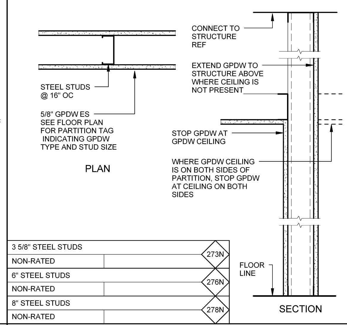
NON-RATED UL NO. C1
