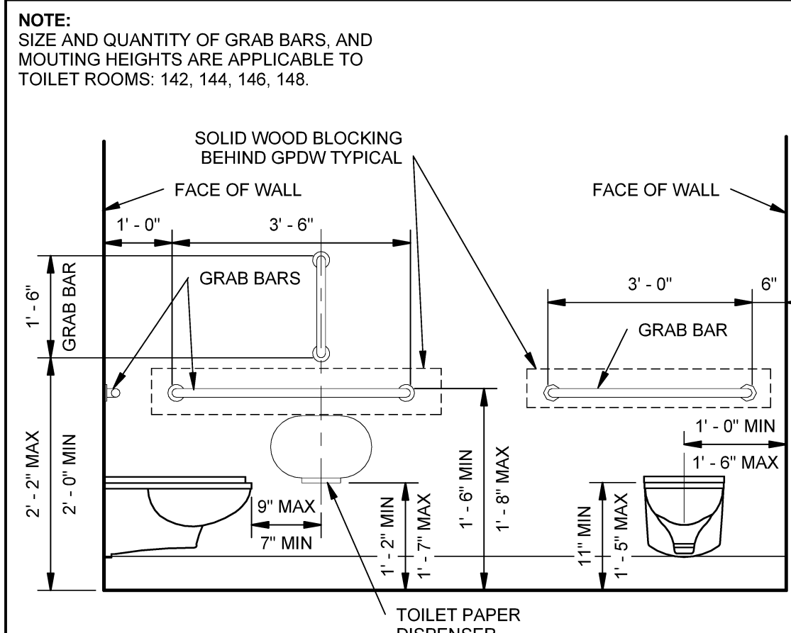
E1 MOUNTING DETAILS AT CHILD RESTROOMS SCALE: 1/2" = 1'-0"
