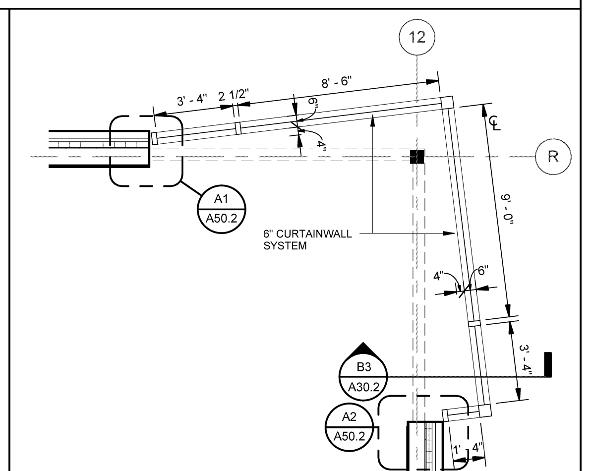
B6 PLAN SECTION AT COLUMN R12 SCALE: 1/4" = 1'-0"
