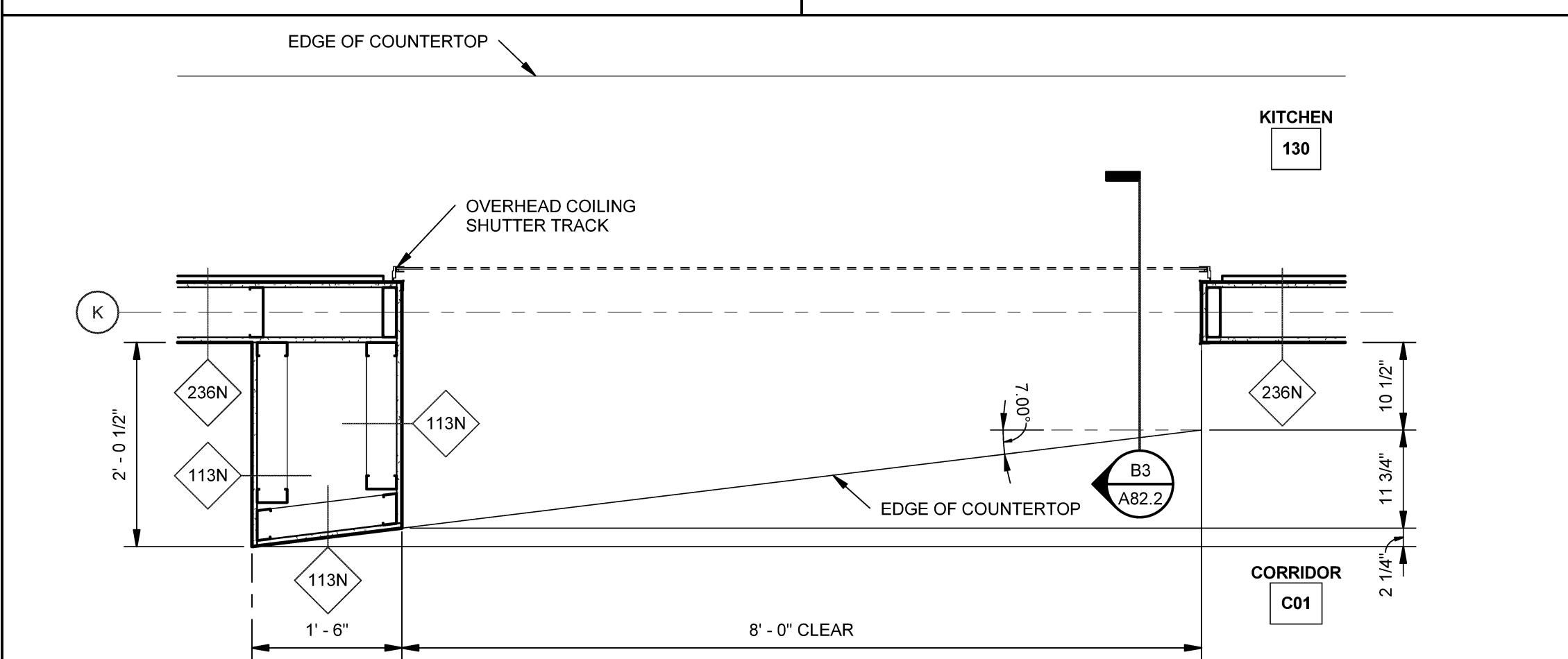
A4 PLAN DETAIL AT SERVING WINDOW SCALE: 3/4" = 1'-0"
