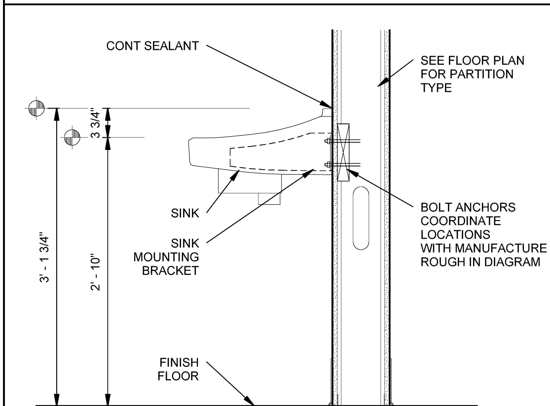
E1 MOUNTING DETAILS AT CHILD RESTROOMS SCALE: 1/2" = 1'-0"
