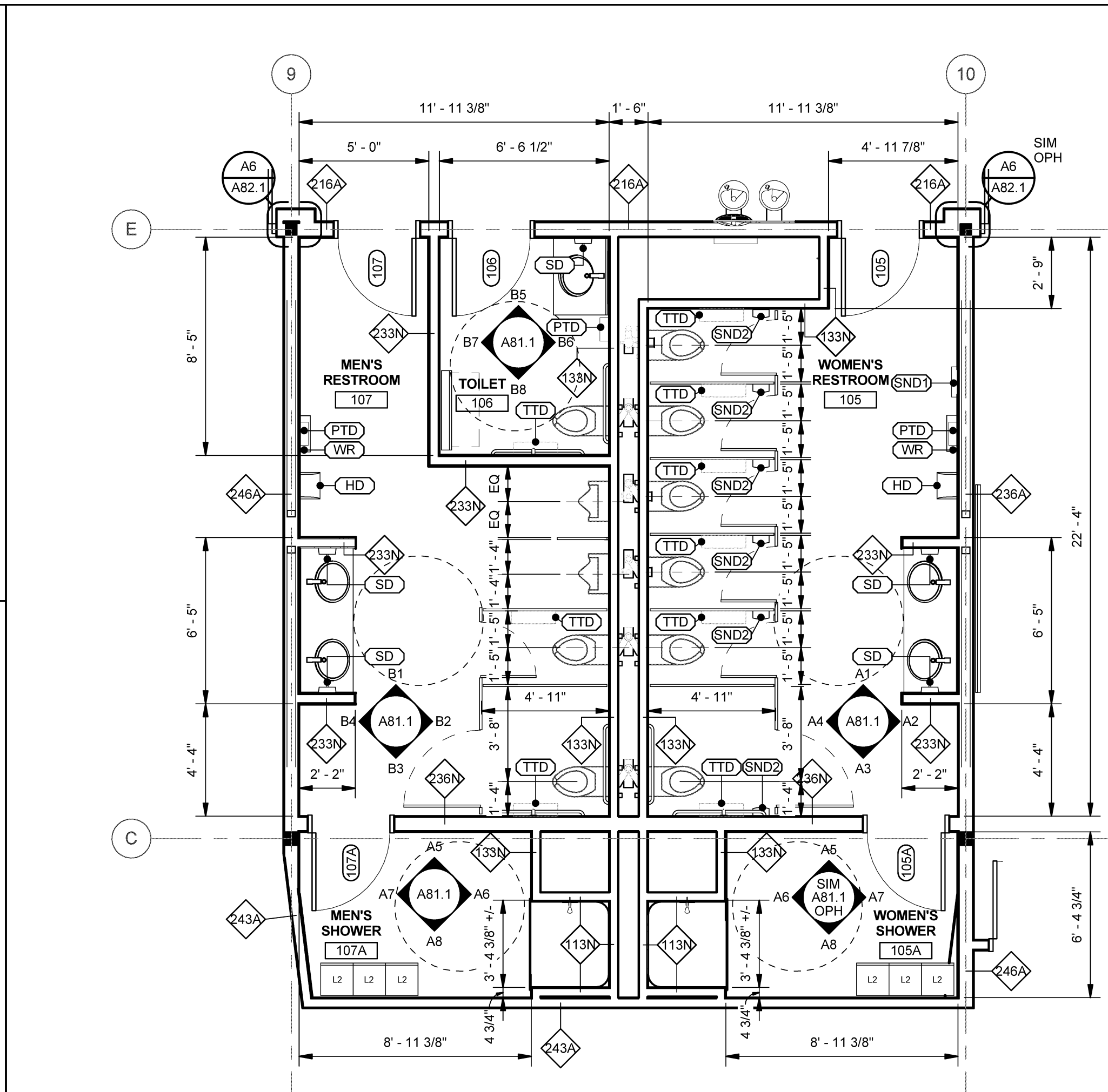
C5 TOILET ROOMS 105 AND 107 SCALE: 1/4" = 1'-0"
