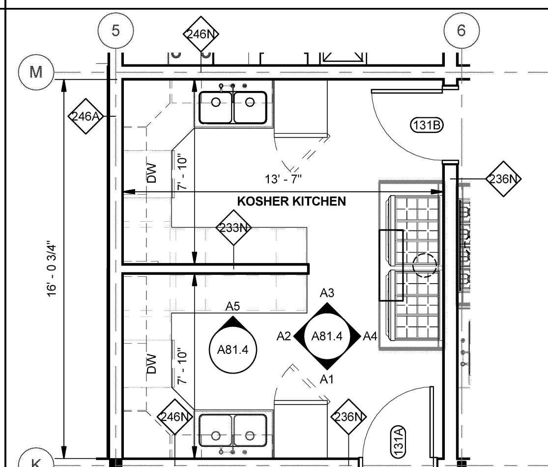
B5 KOSHER KITCHEN ENLARGED PLAN SCALE: 1/4" = 1'-0"
