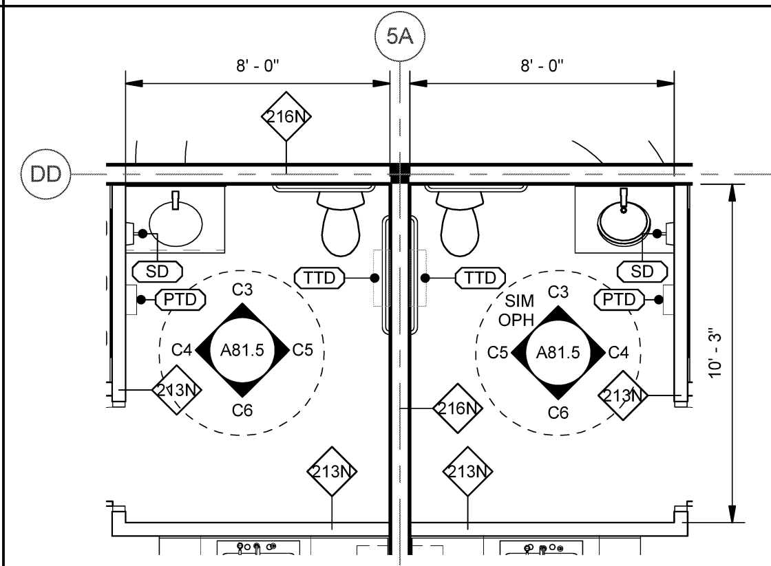
E2 MOUNTING DETAILS SCALE: 1/2" = 1'-0"
