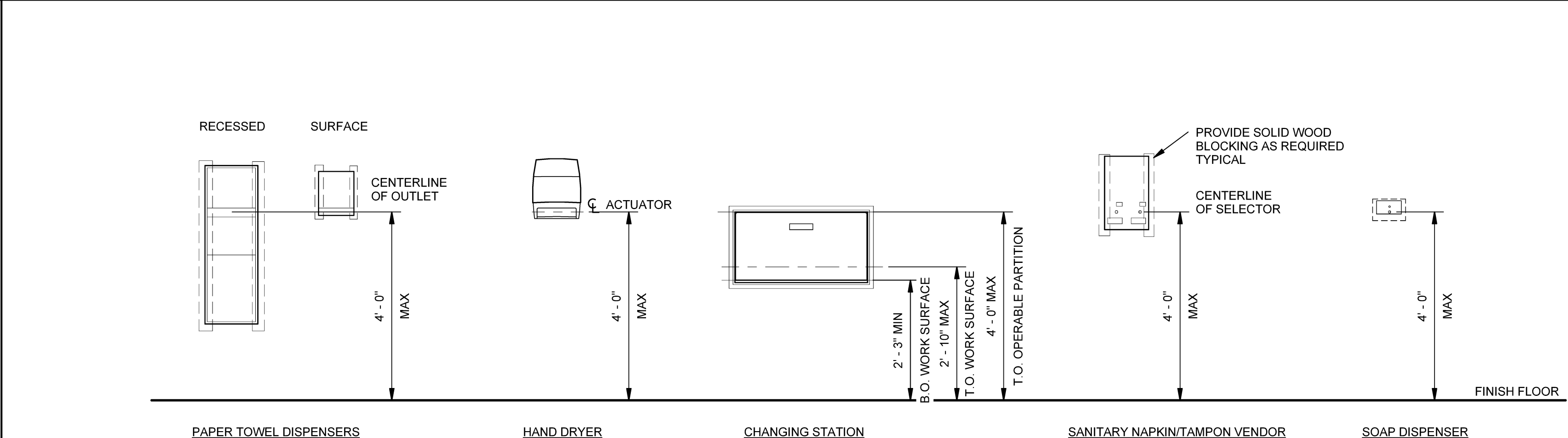
E4 DISPENSER MOUNTING HEIGHTS SCALE: 1/2" = 1'-0"
