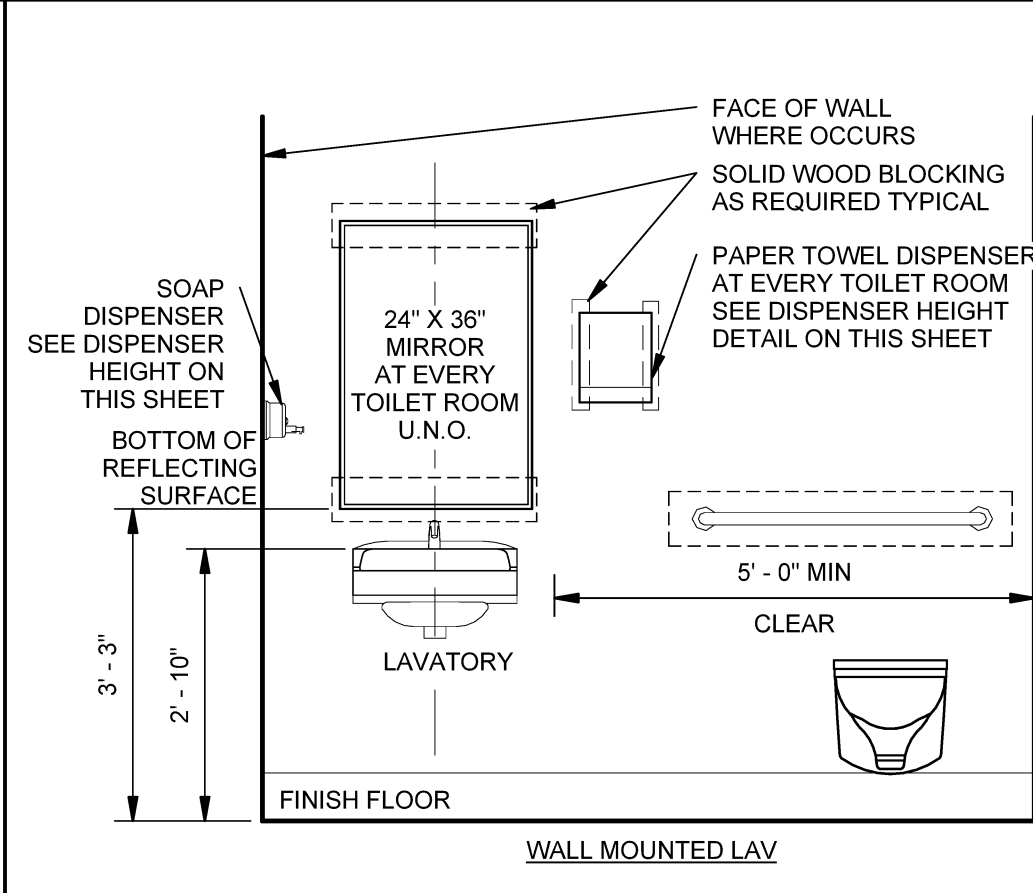
E3 LAVATORY MOUNTING HEIGHTS SCALE: 1/2" = 1'-0"
