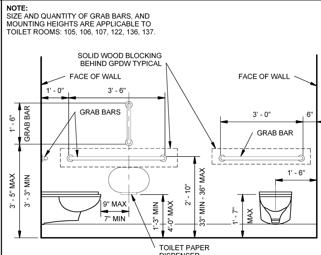
E2 MOUNTING DETAILS SCALE: 1/2" = 1'-0"
