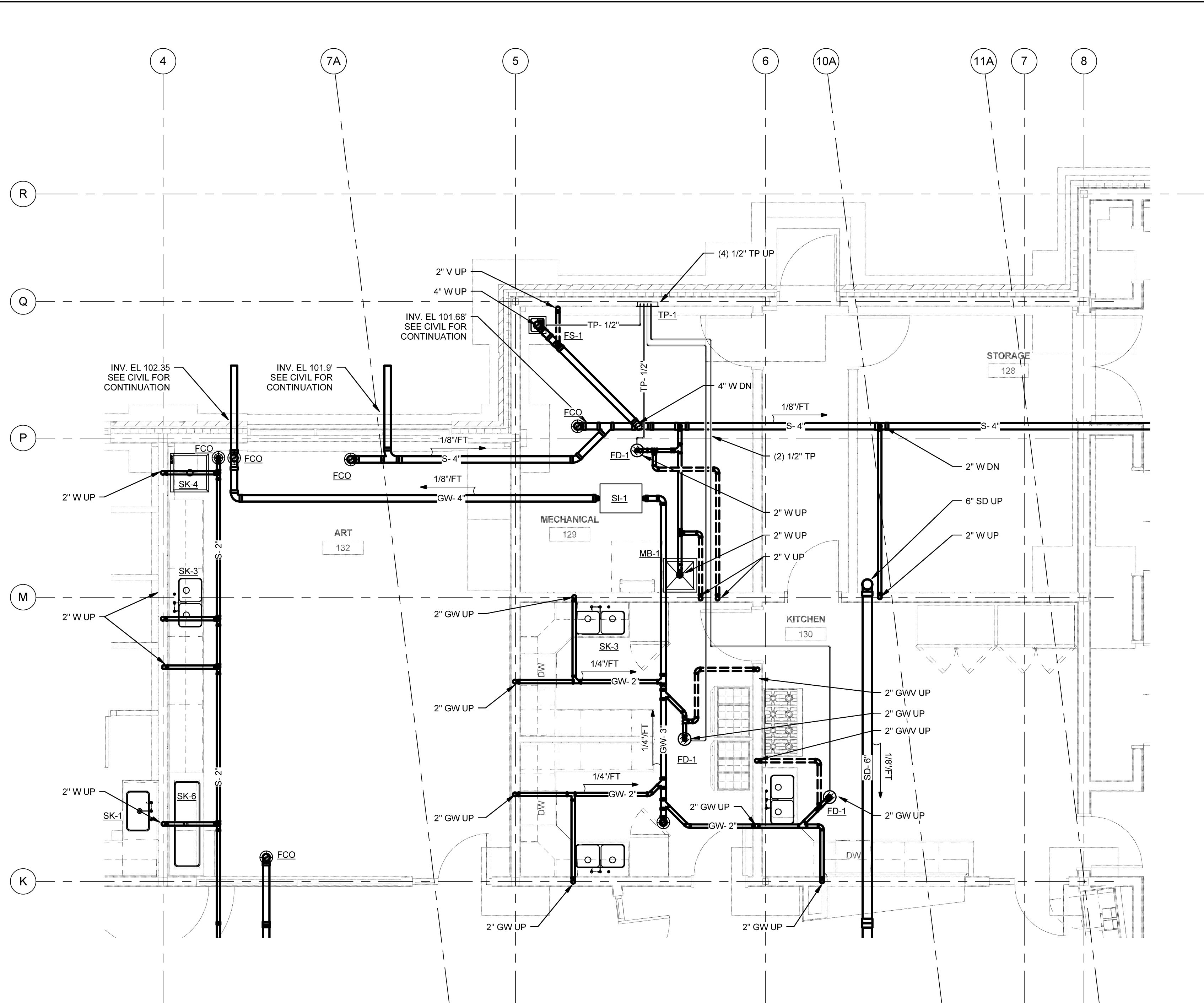
1 BELOW SLAB DRAINAGE SCALE: 1/4" = 1'-0"
