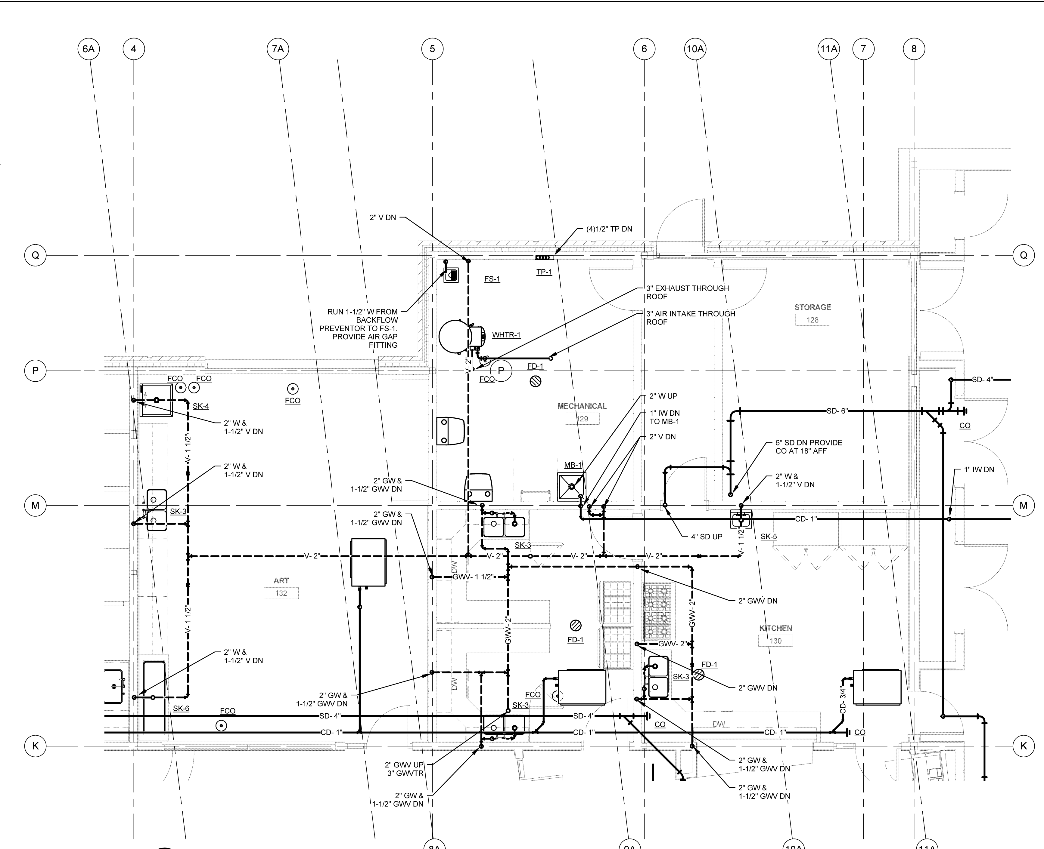
2 ABOVE SLAB DRAINAGE SCALE: 1/4" = 1'-0"
