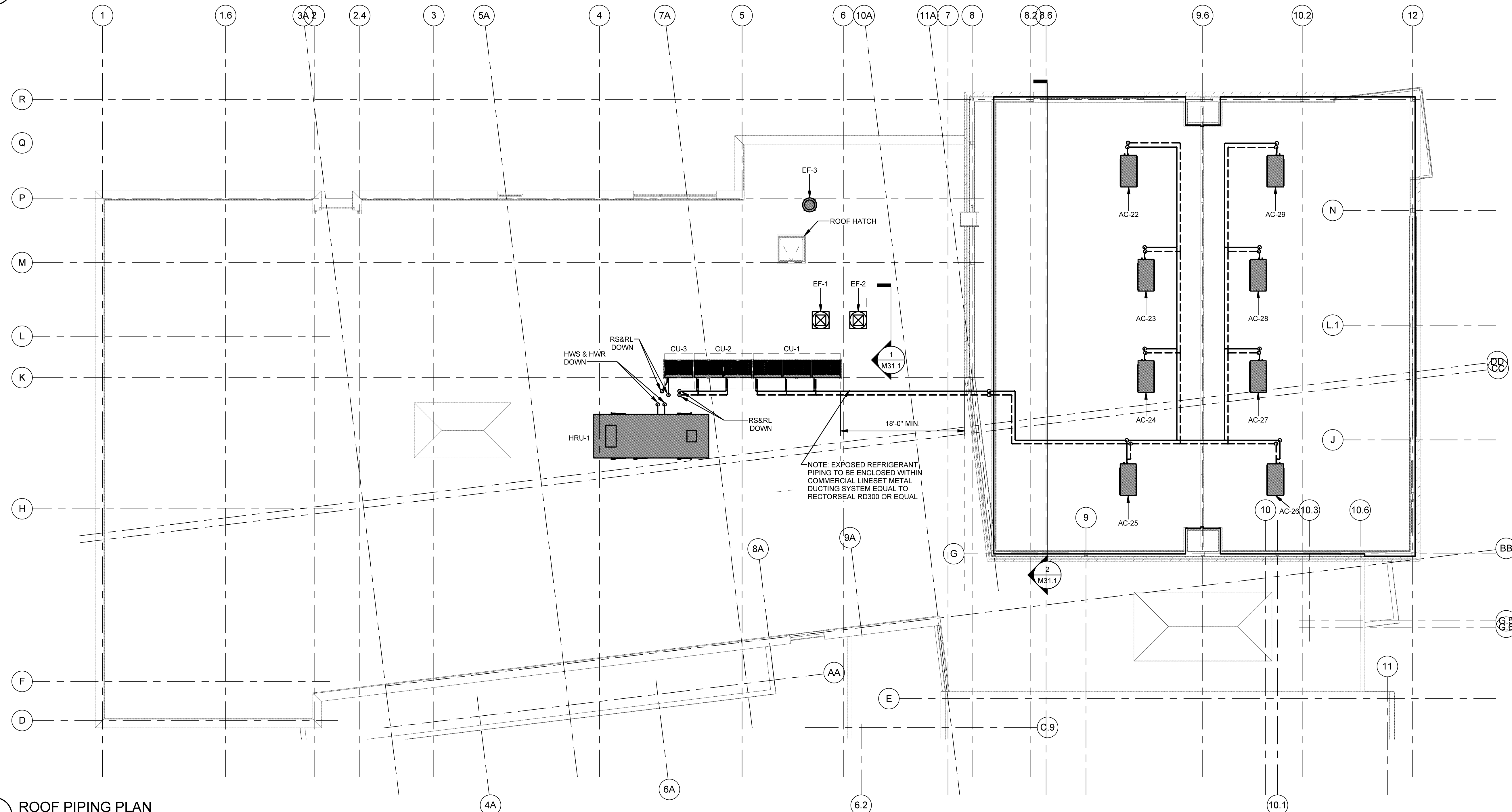
1 ROOF PIPING PLAN
