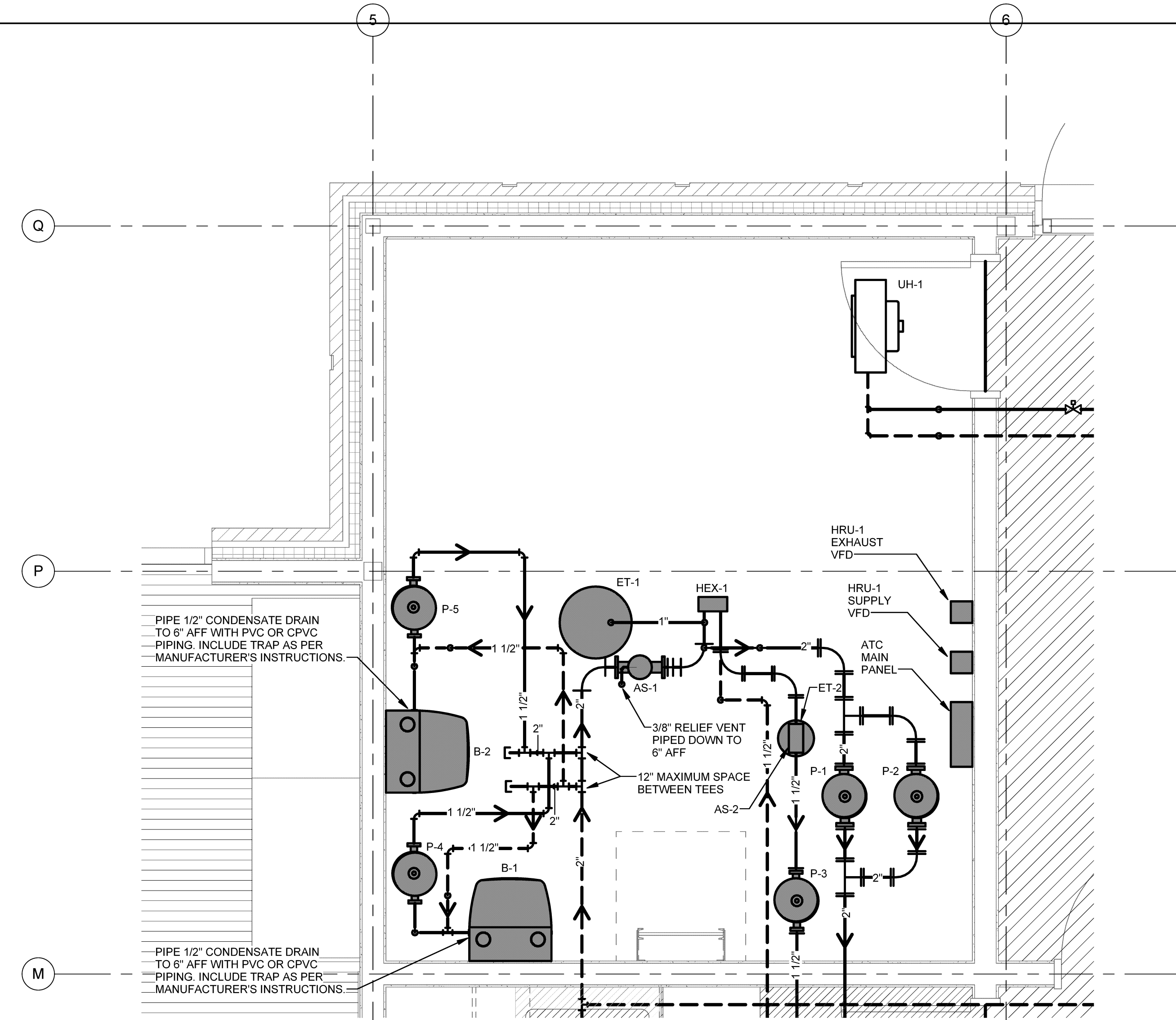
2 MECHANICAL ROOM PART PLAN
