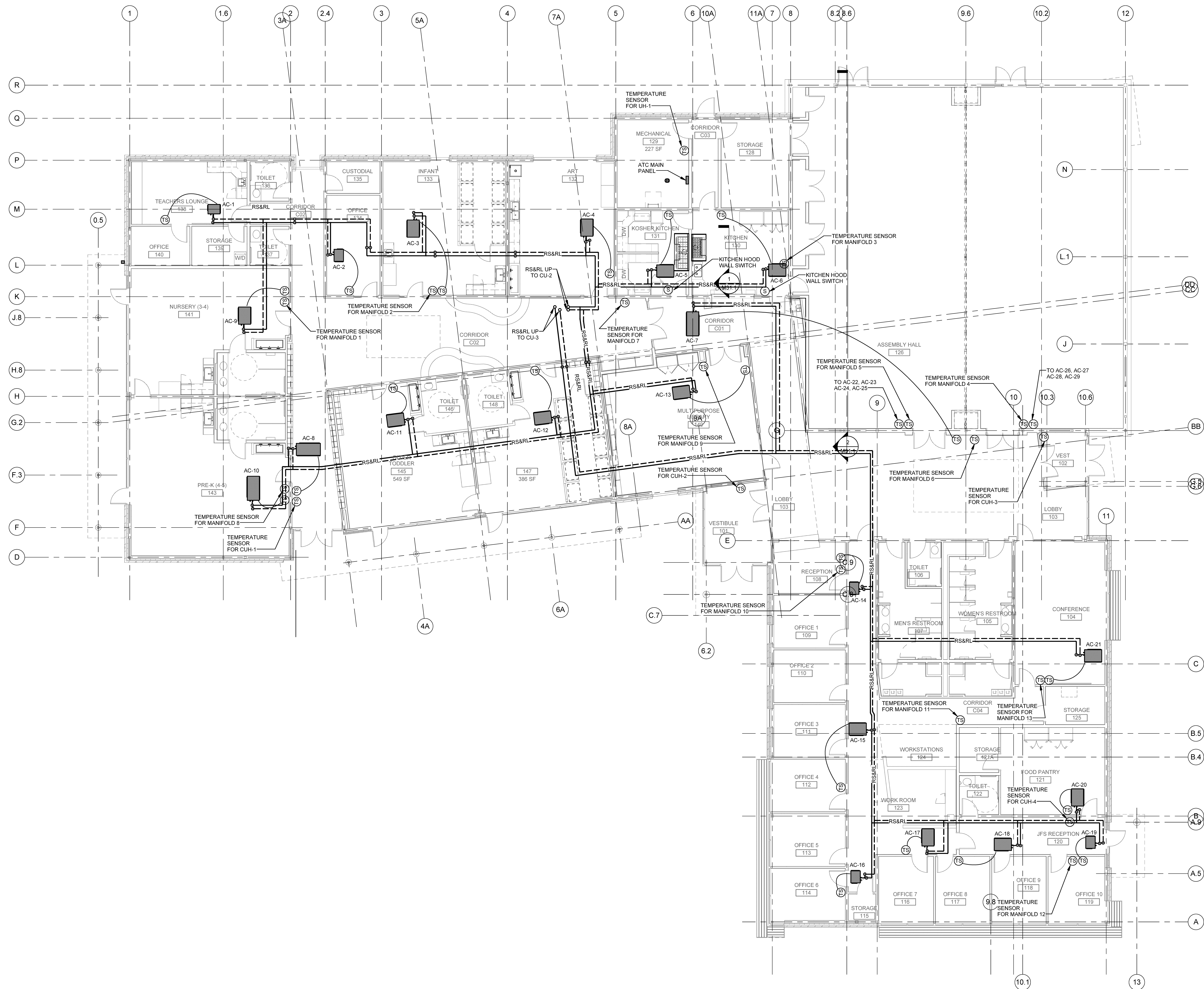
1 FIRST FLOOR PIPING PLAN SCALE: 1/8" = 1'-0"
