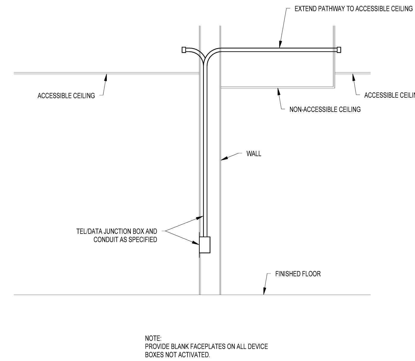
7 TYPICAL WALL OUTLET DETAIL SCALE: 1/8" = 1'-0"
