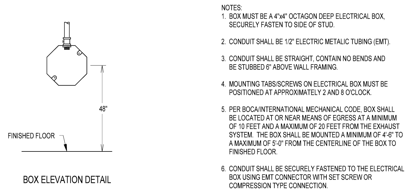
12 ANSUL SYSTEM MANUAL PULL BOX DETAIL NO SCALE
