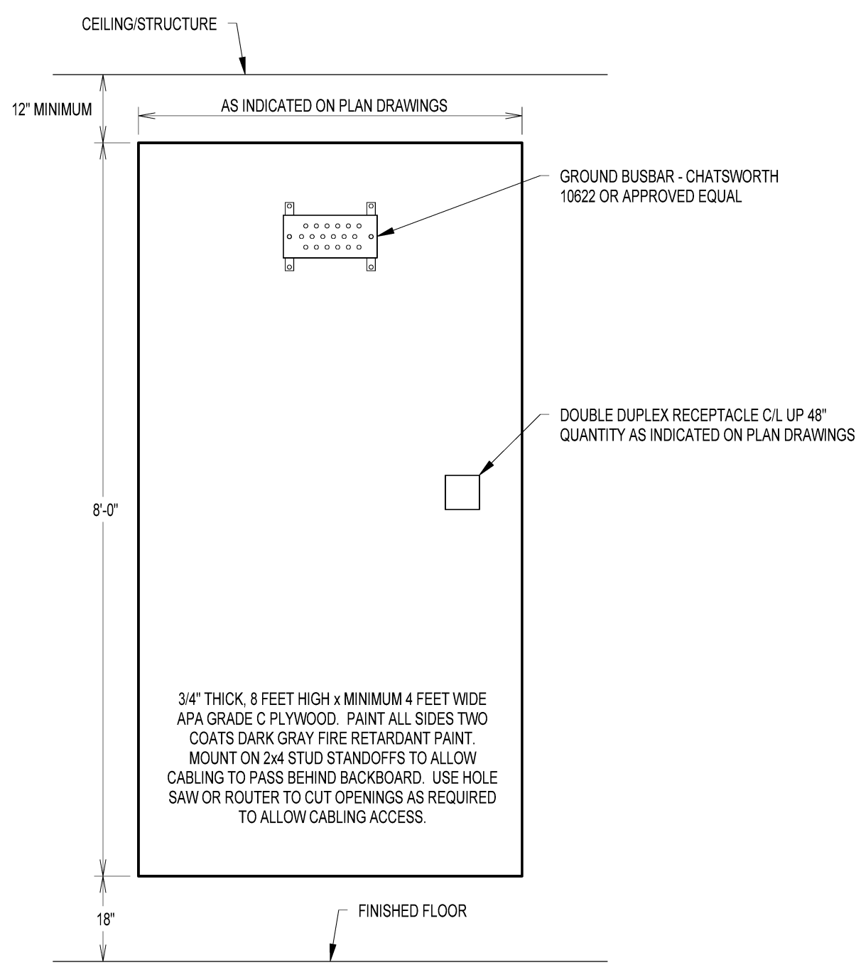
6 TYPICAL TLE/DATA BACKBOARD (BKBD) SCALE: 1/8" = 1'-0"
