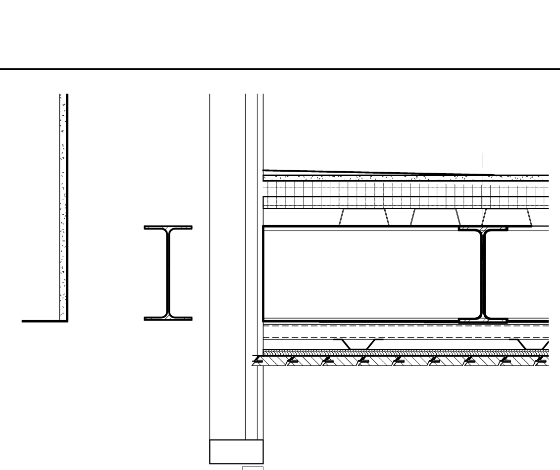
C3 SECTION AT LOBBY - Callout 1 SCALE: 1 1/2" = 1'-0"
