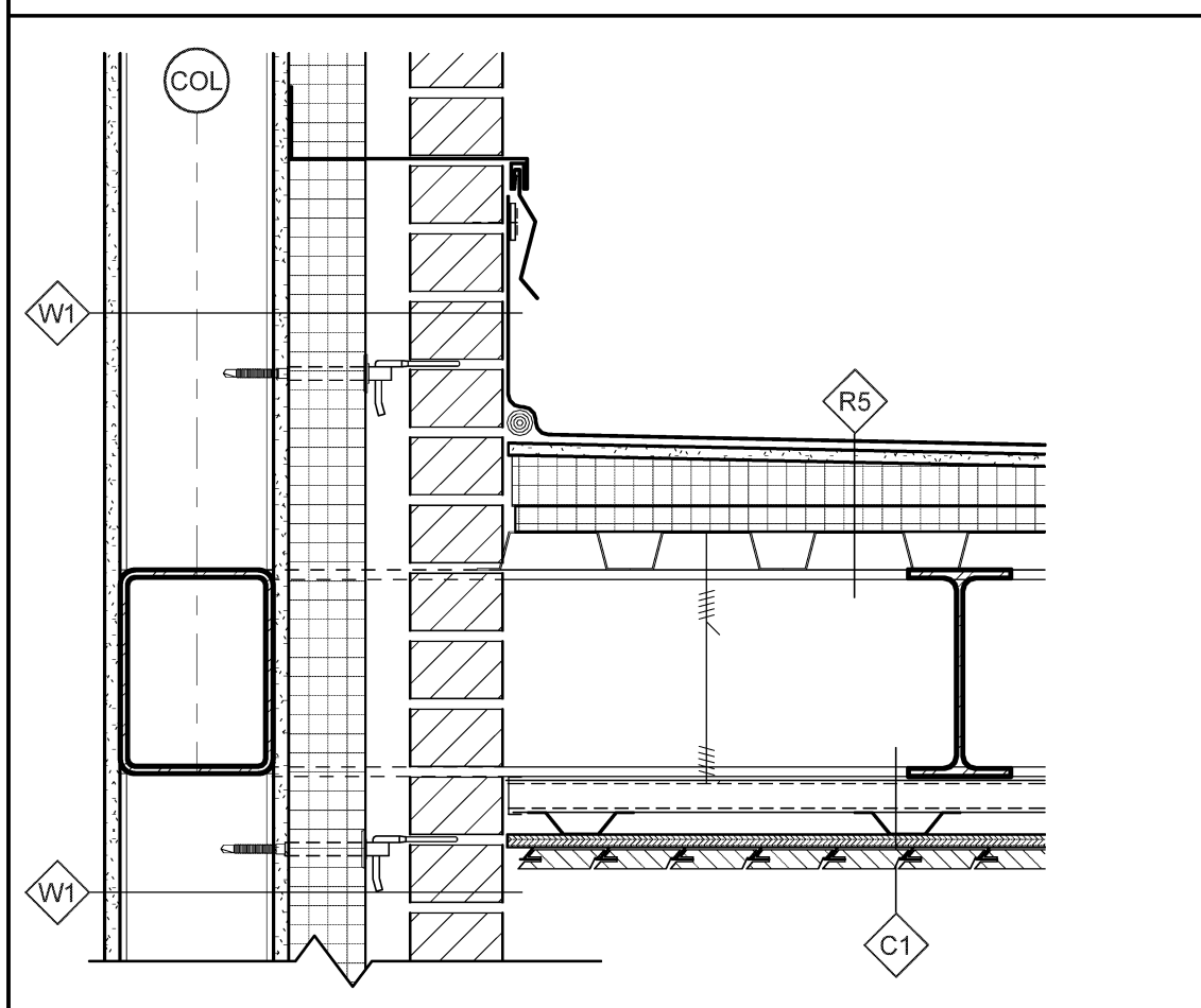
D1 DETAIL AT ENTRY CANOPY SCALE: 1 1/2" = 1'-0"
