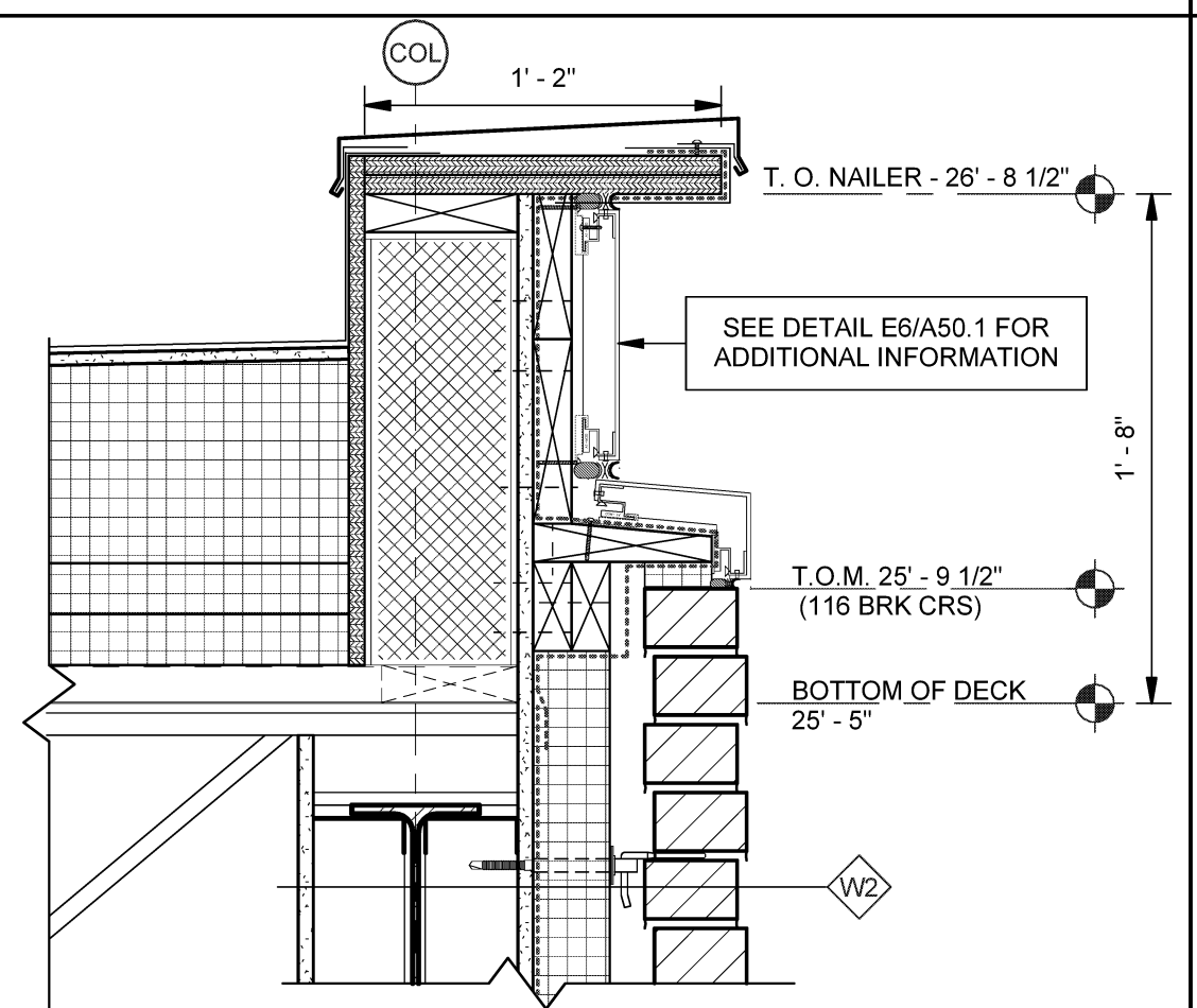
D5 ROOF EDGE AT ASSEMBLY ROOF SCALE: 1 1/2" = 1'-0"
