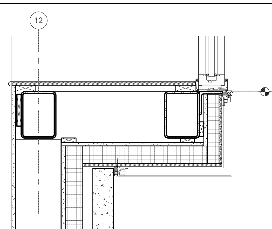
D2 DETAIL AT ASSEMBLY WINDOW SCALE: 1 1/2" = 1'-0"
