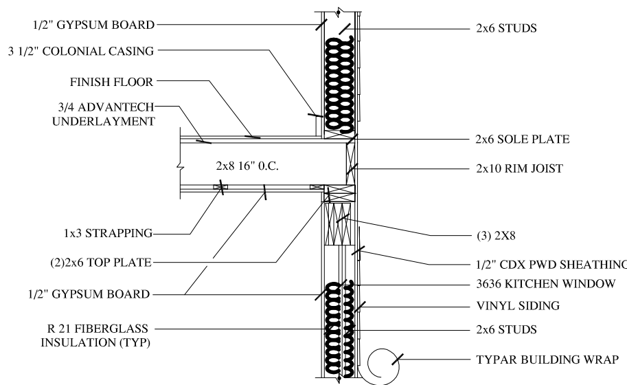
EXTERIOR WALL DETAIL
