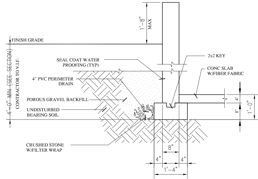
FOOTING DETAIL
