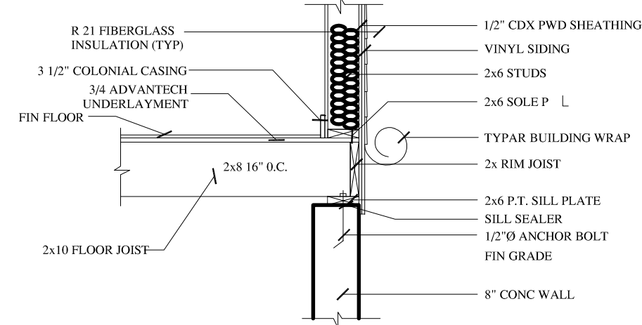
WALL BASE DETAIL
