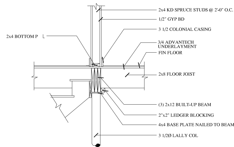
COLUMN/GIRDER DETAIL
