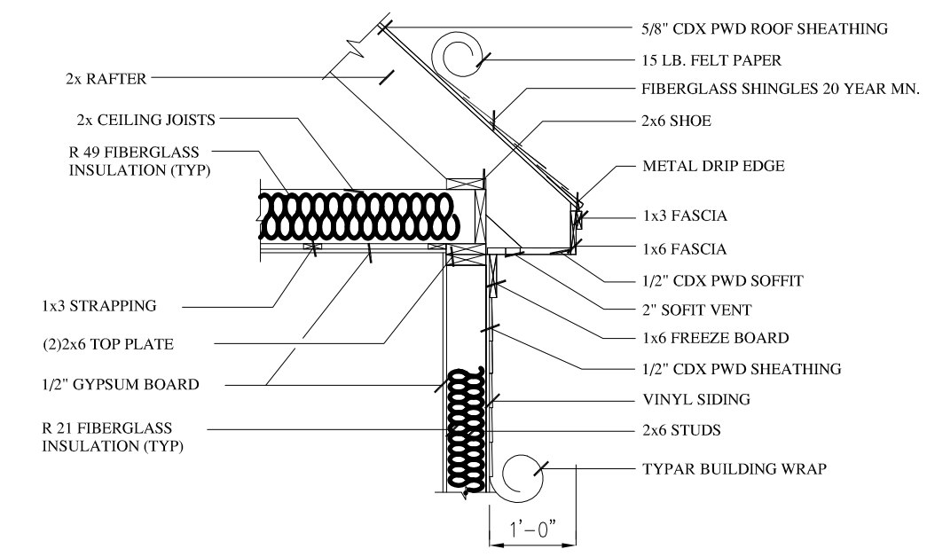
SOFFIT DETAIL
