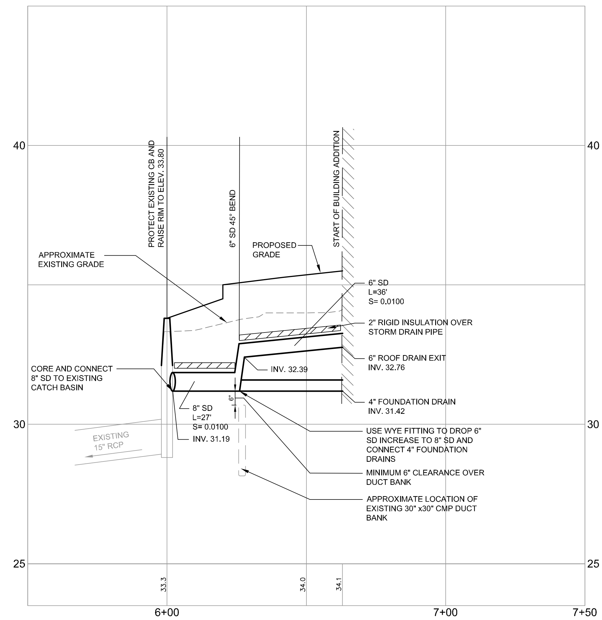
8" AND 6" STORM DRAIN PROFILE 1" = 20' HORIZ. 1" = 2' VERT.
