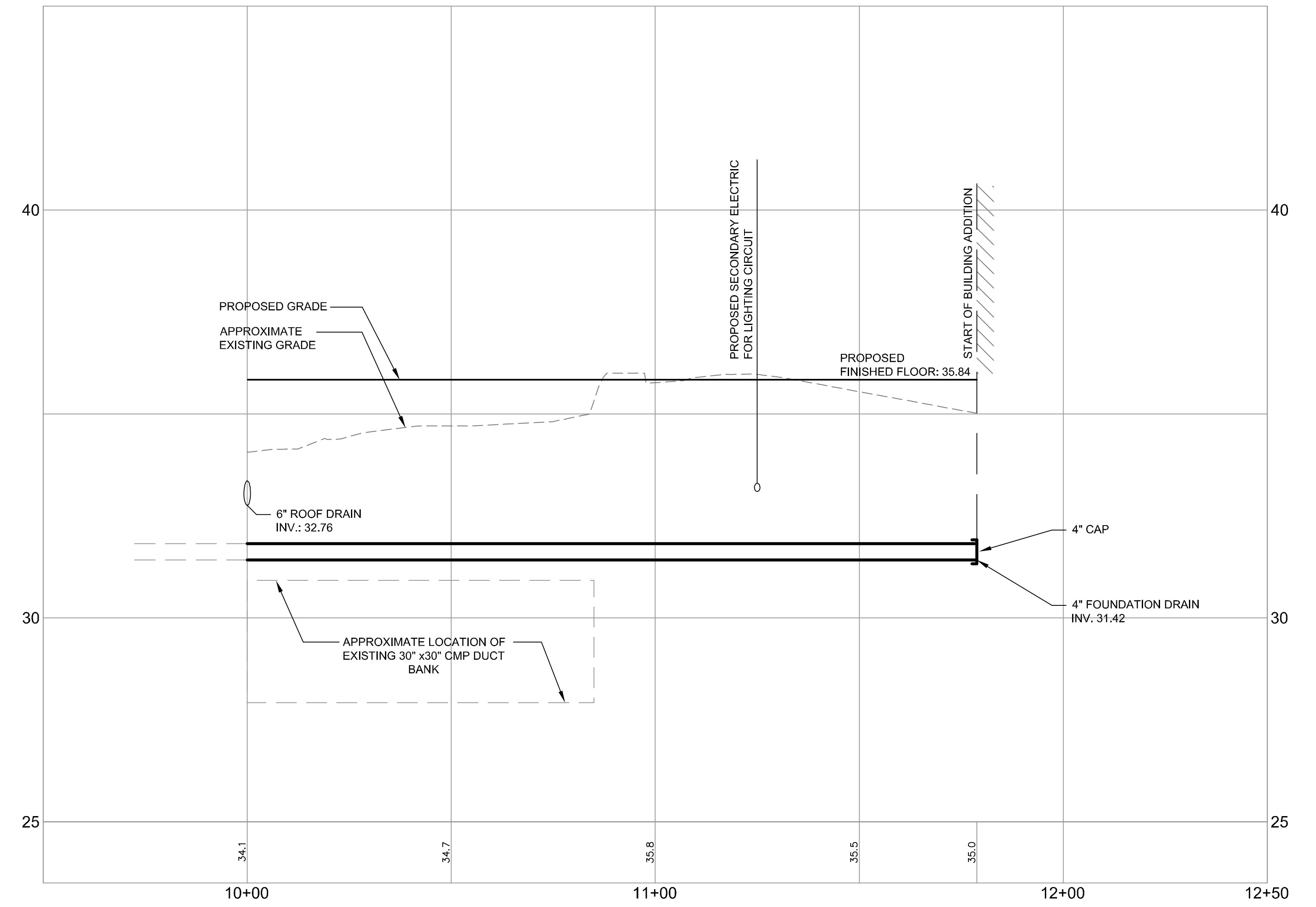
4" FOUNDATION DRAIN PROFILE 1" = 20' HORIZ. 1" = 2' VERT.
