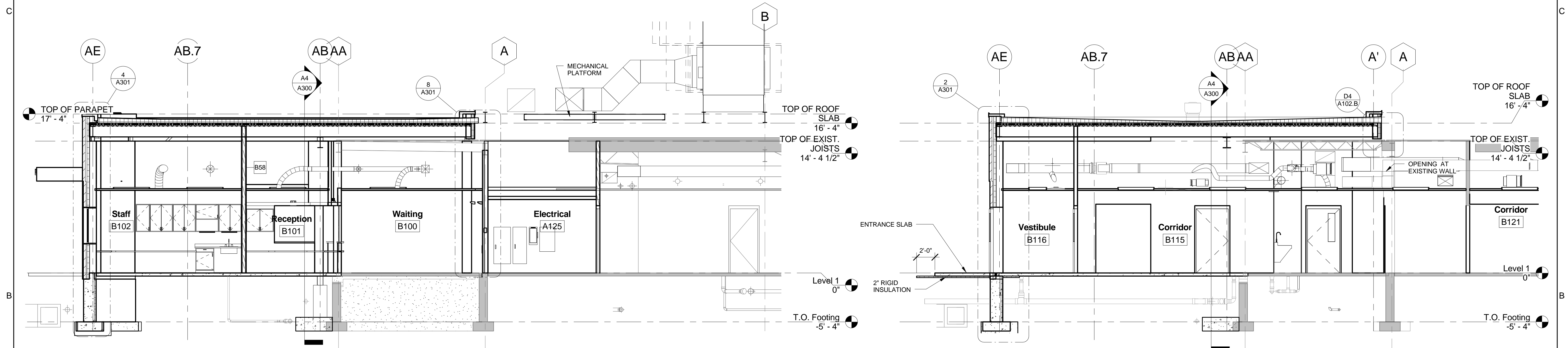
B5 Section at A&B Additions - Through Waiting B100 3/16" = 1'-0"
