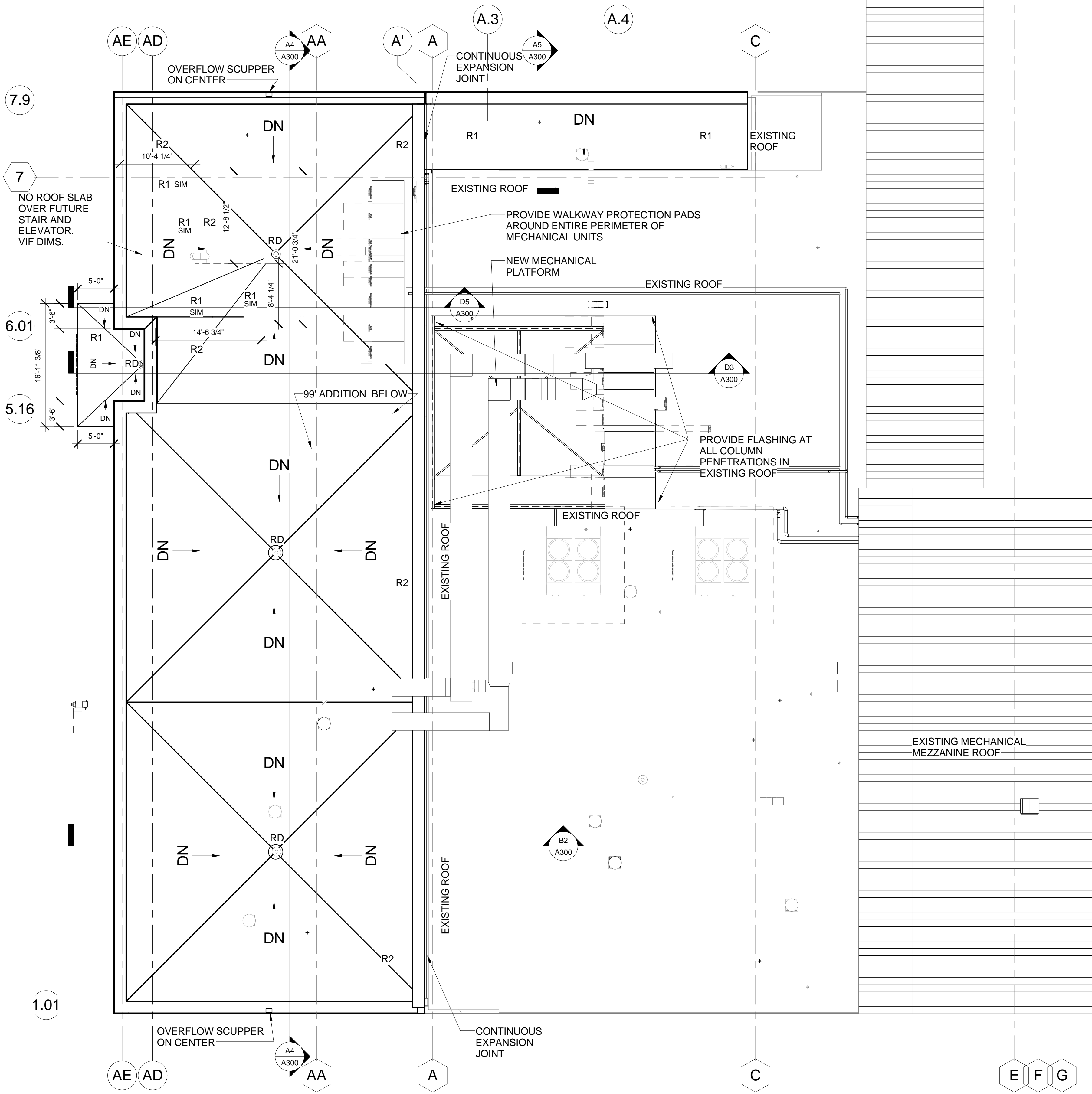
A2 Roof Plan 1/8" = 1'-0"
