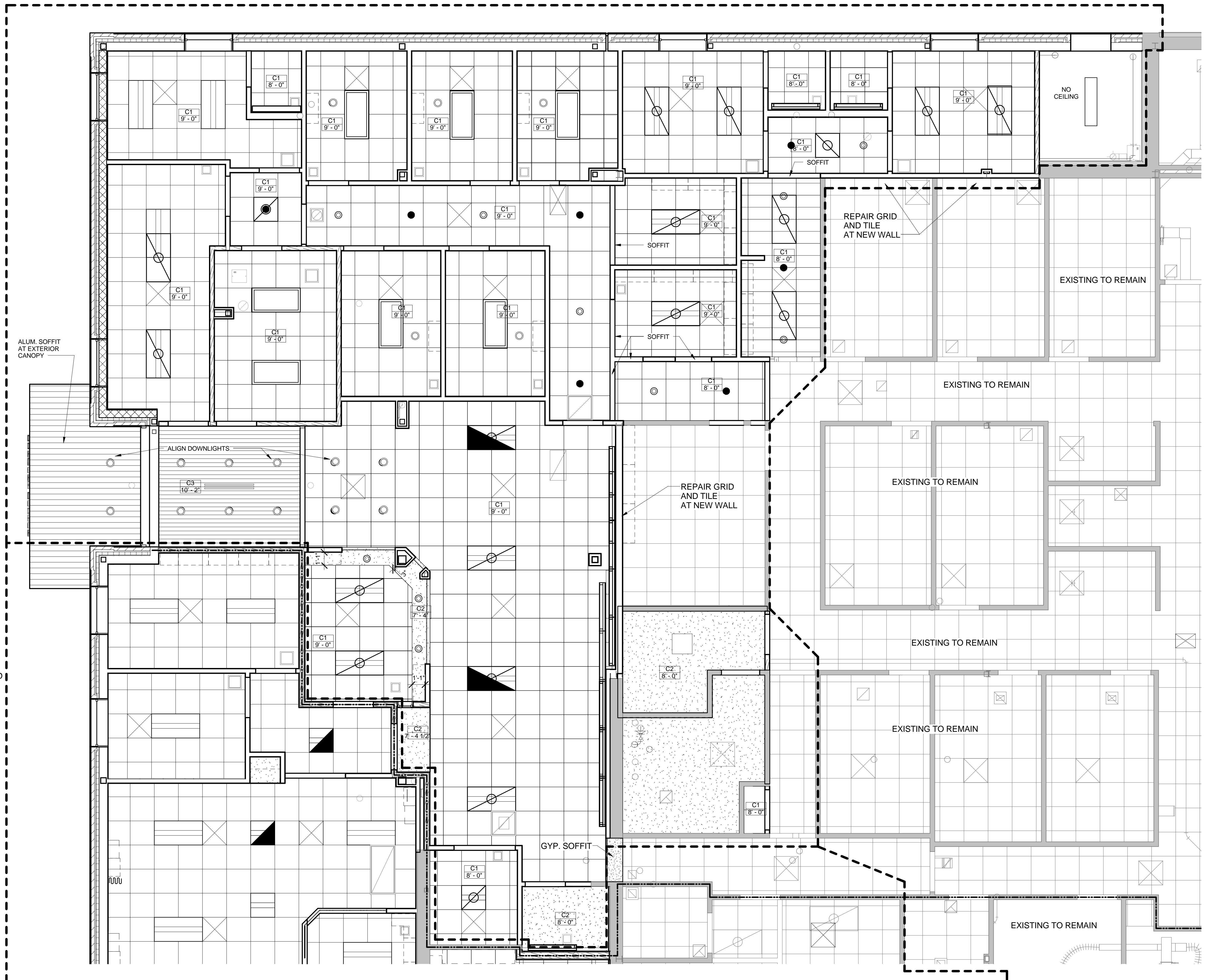
A4 CEILING PLAN "A" 1/4" = 1'-0"
