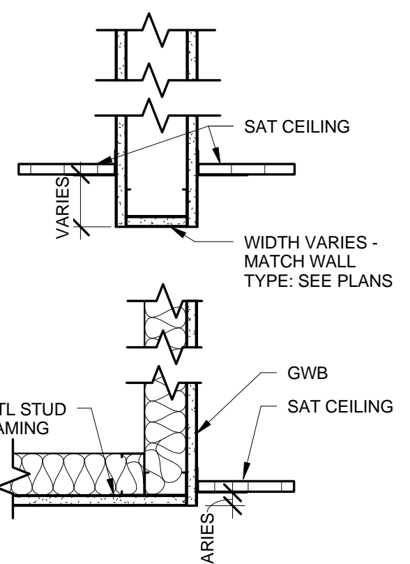
D5 TYPICAL CEILING DETAILS 1 1/2" = 1'-0"
