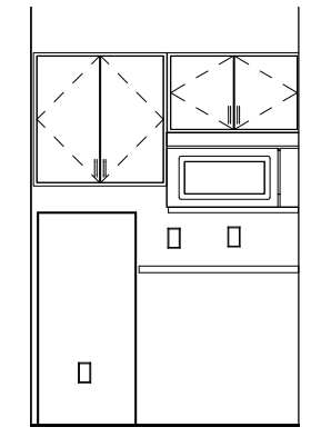
③ Elevation 1 - d 1/4" = 1'-0"
