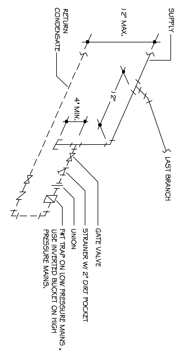
END OF MAIN DRIP DETAIL
