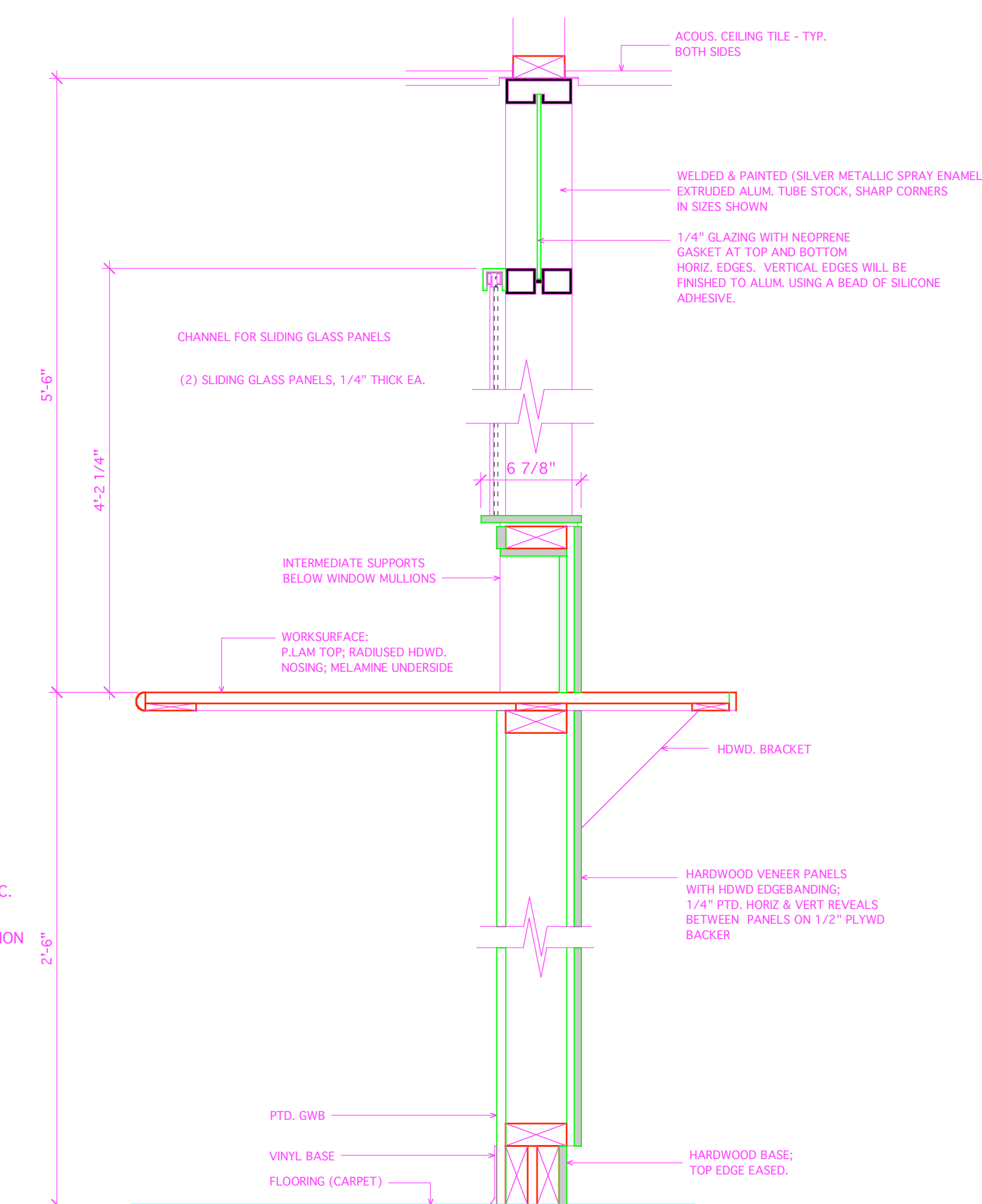
2 SECTION @ P.T. RECEPTION 162 A-702 SCALE: 1 1/2" = 1'-0"
