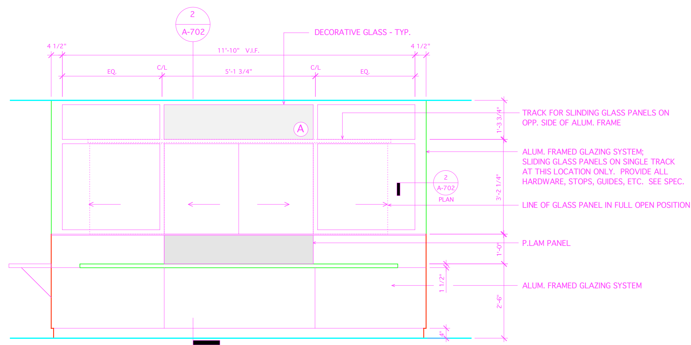
5 ELEVATION OF GLASS WALL/COUNTER @ P.T. RECEPTION 162 A-702 SCALE: 1/2" = 1'-0"
