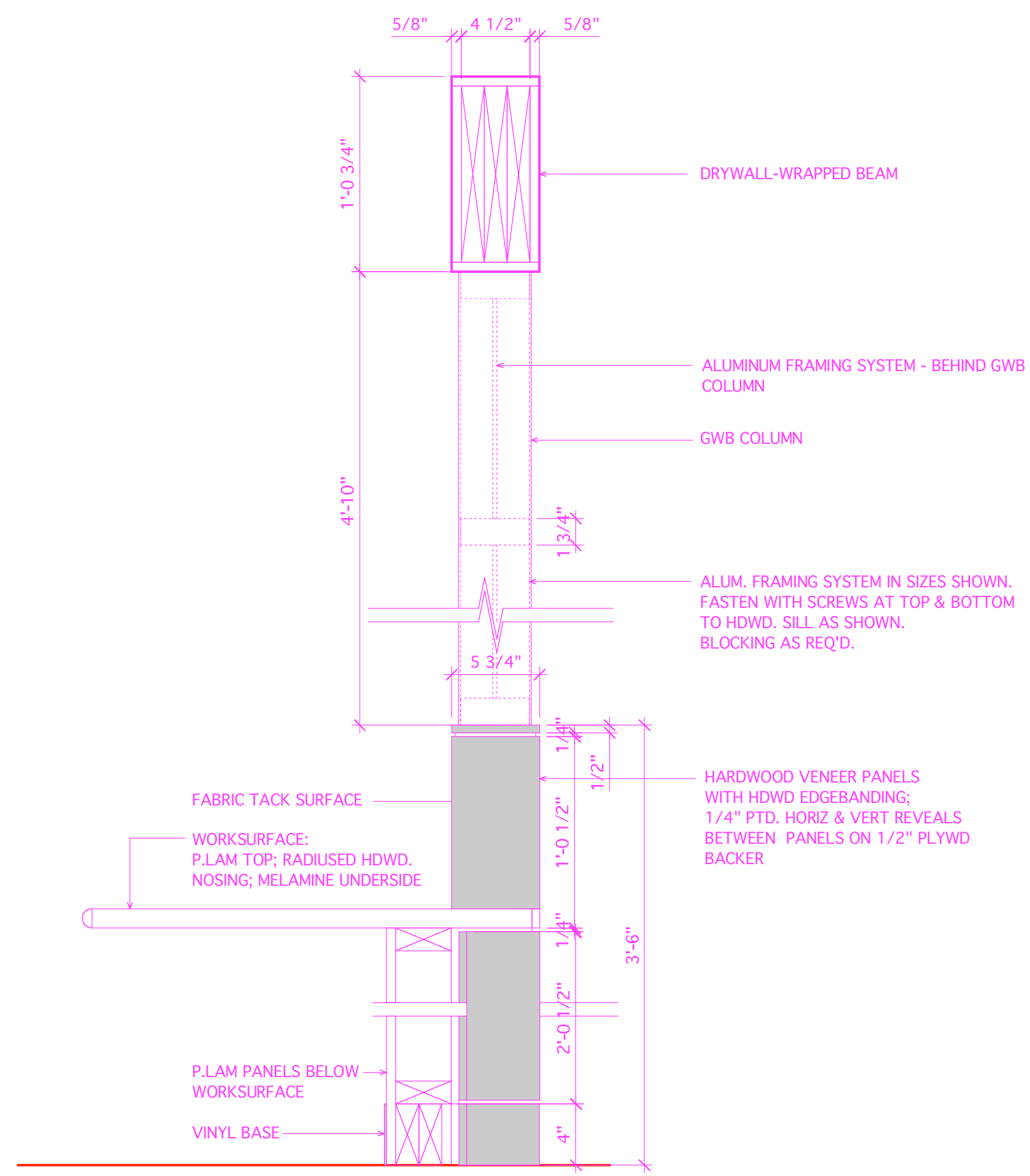
9 DTL. THROUGH RECEPTION OPENING - LOBBY 100 A-702 SCALE: 1 1/2" = 1'-0"
