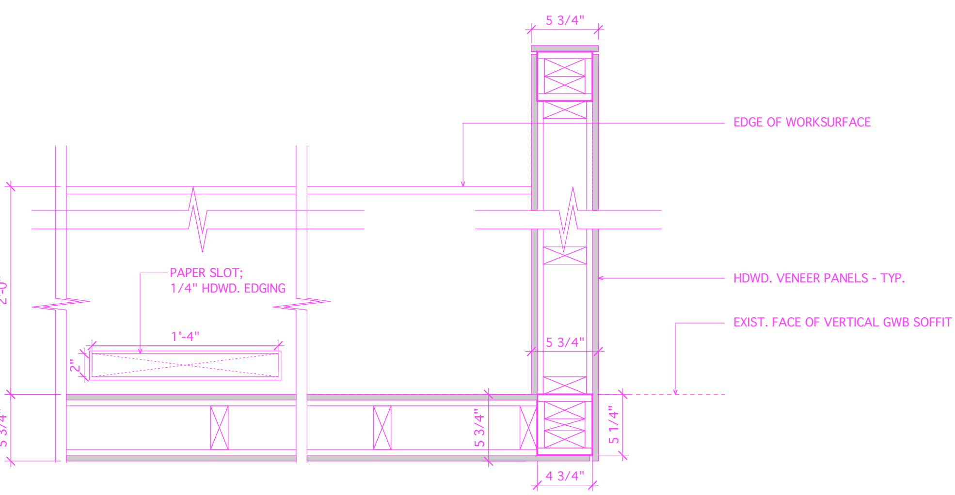
11 PLAN DTL. @ PANELING / COPIER COUNTER - LOBBY 100 A-702 SCALE: 1 1/2" = 1'-0"
