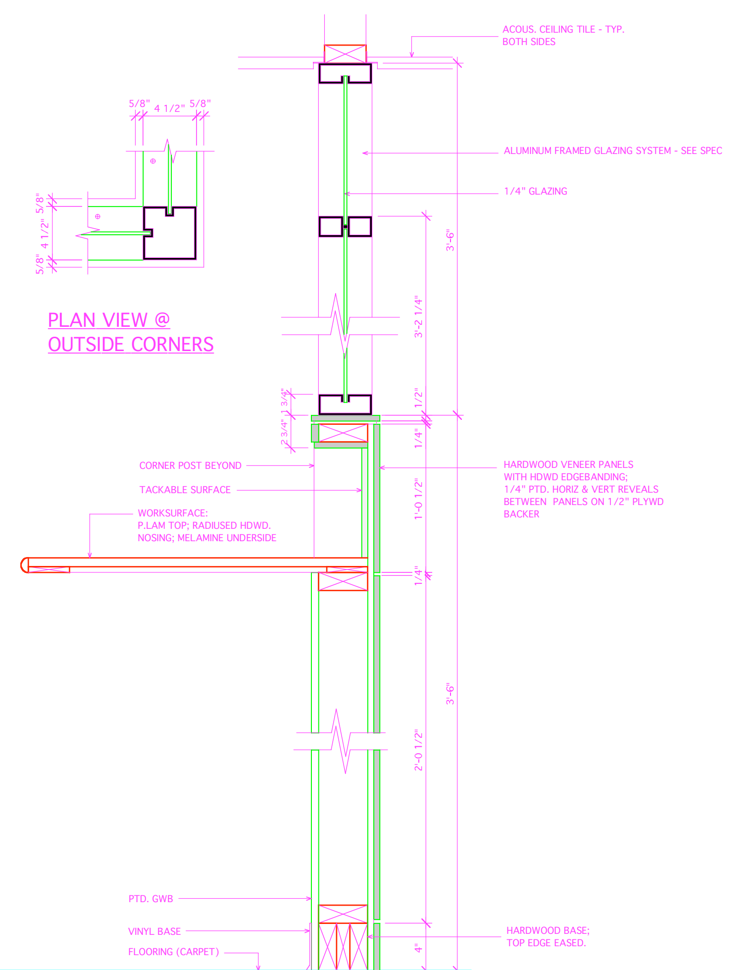
1 SECTION @ P.T. RECEPTION 162 A-702 SCALE: 1 1/2" = 1'-0"
