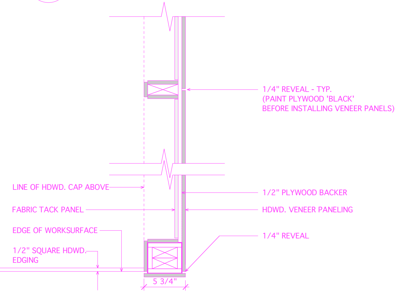
8 DTL. @ VENEER paneled WALL - LOBBY 100 A-702 SCALE: 1 1/2" = 1'-0"
