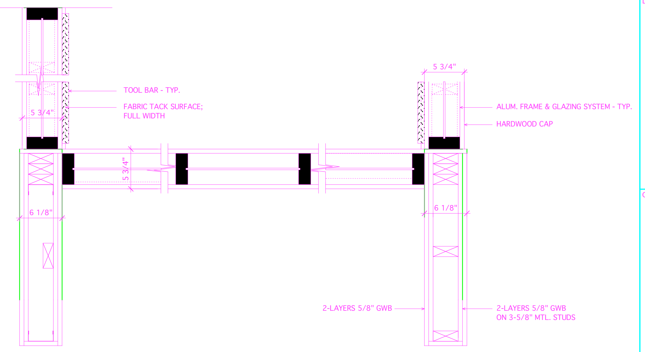
12 DTL. @ GWB-WRAPPED VERTICAL SUPPORT - LOBBY 100 A-702 SCALE: 1 1/2" = 1'-0"
