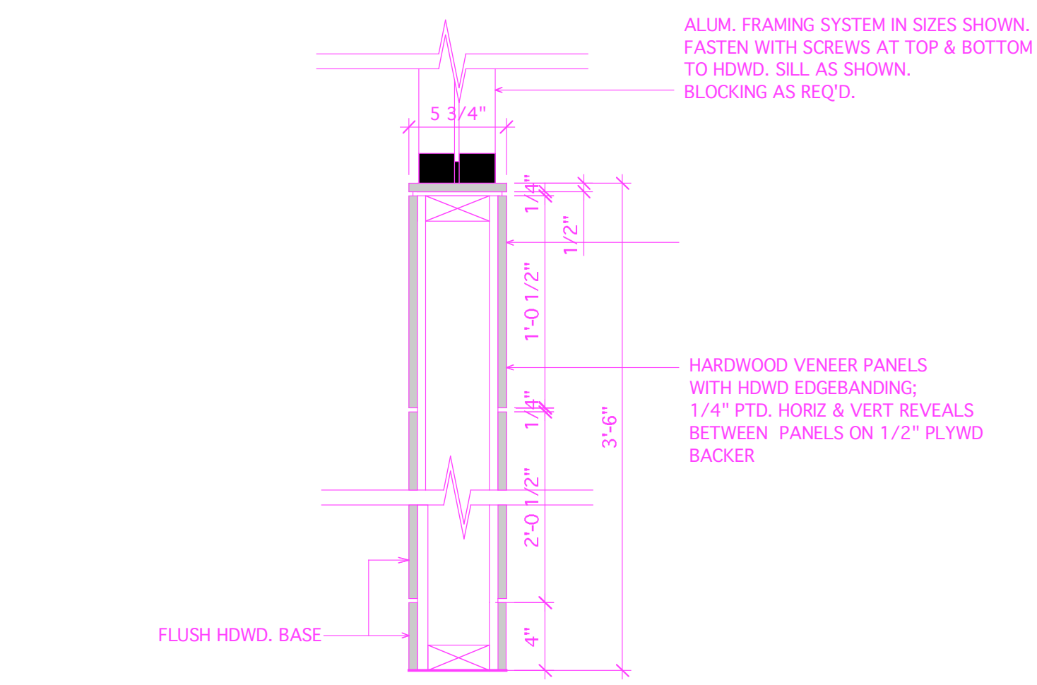
8 DTL. @ VENEER paneled WALL - LOBBY 100 A-702 SCALE: 1 1/2" = 1'-0"
