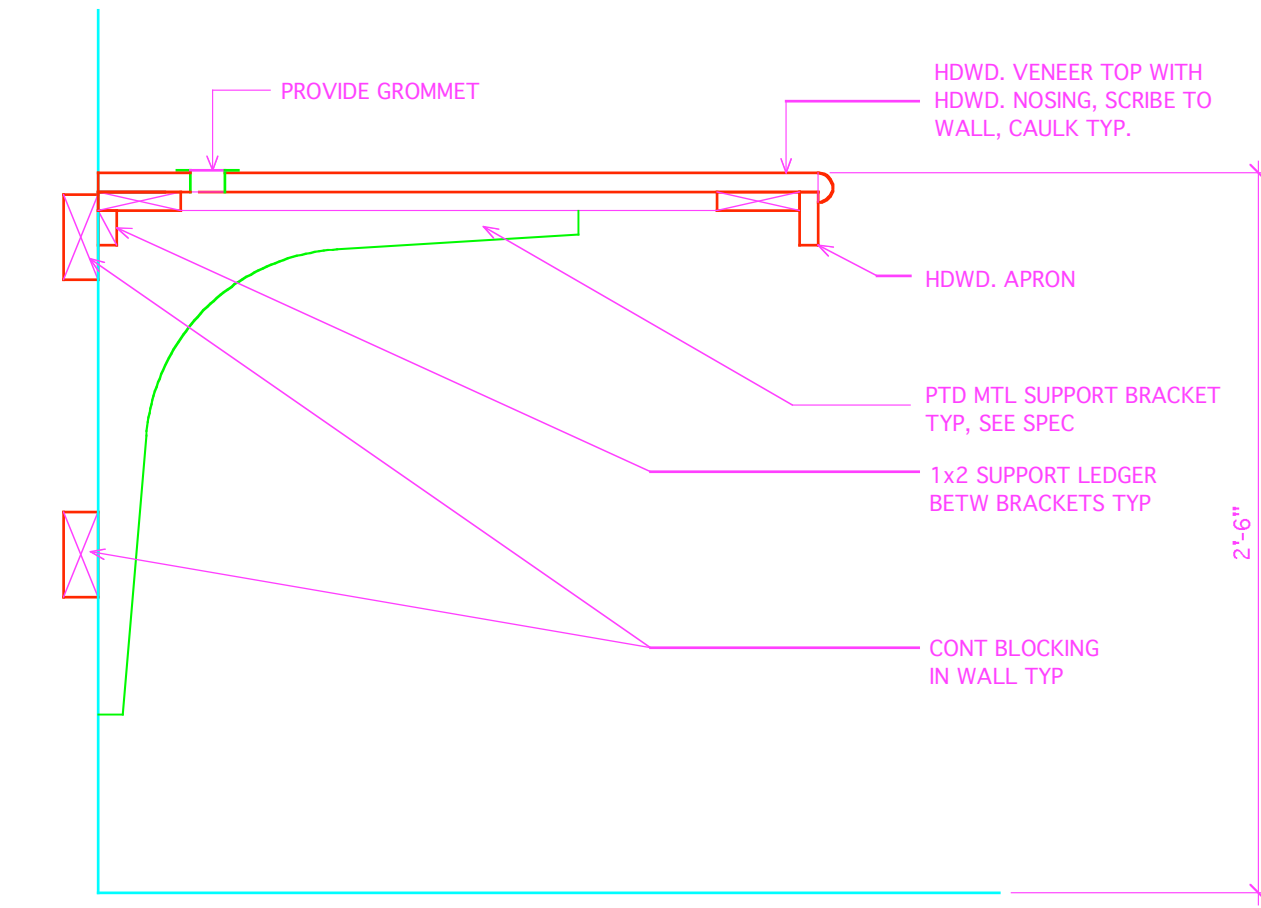
3 COMPUTER COUNTER @ LIBRARY 225 A-702 SCALE: 1 1/2" = 1'-0"
