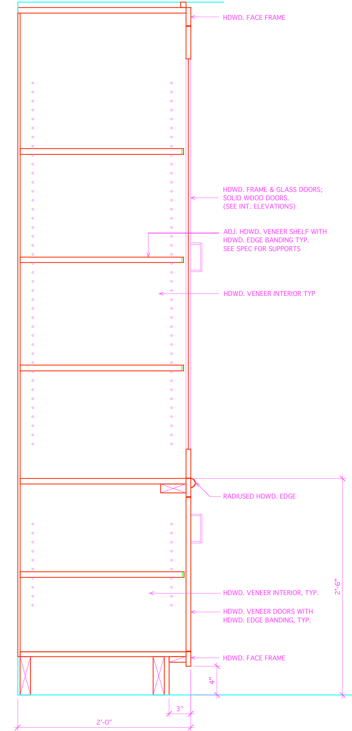
4 CABINET @ LIBRARY 225 A-702 SCALE: 1 1/2" = 1'-0"
