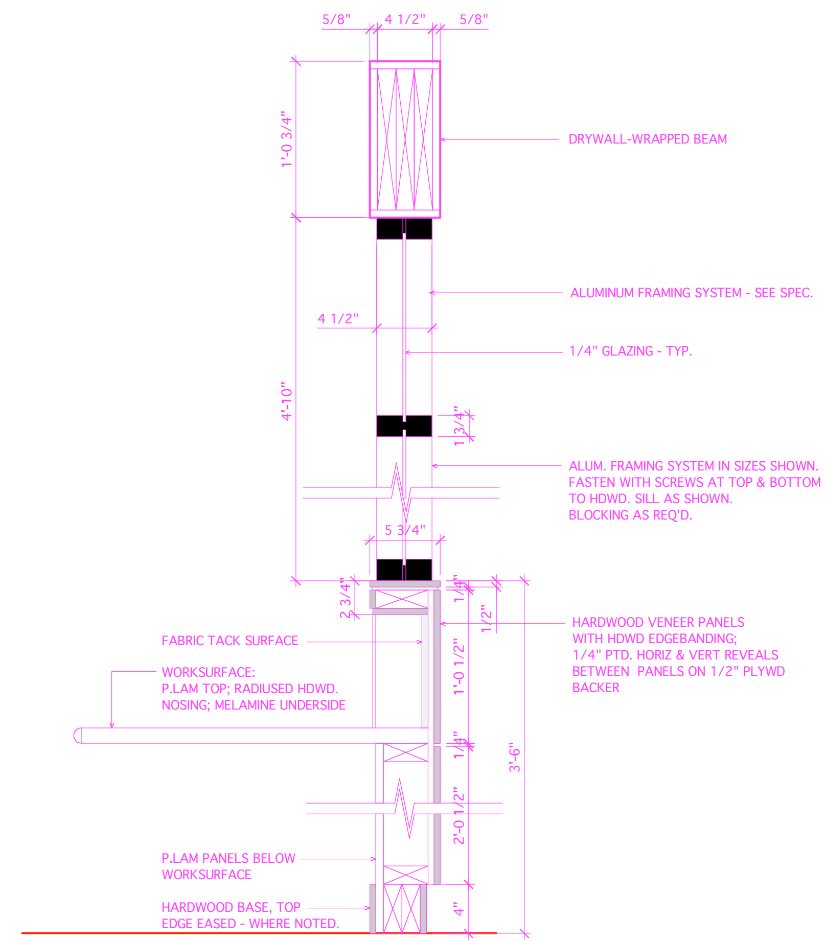
10 DTL. @ GWB-WRAPPED VERTICAL SUPPORT - LOBBY 100 A-702 SCALE: 1 1/2" = 1'-0"
