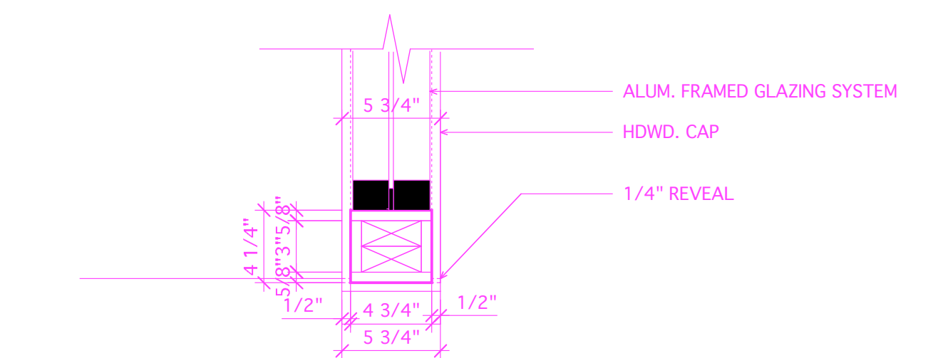
6 DTL. @ GWB-WRAPPED VERTICAL SUPPORT - LOBBY 100 A-702 SCALE: 1 1/2" = 1'-0"
