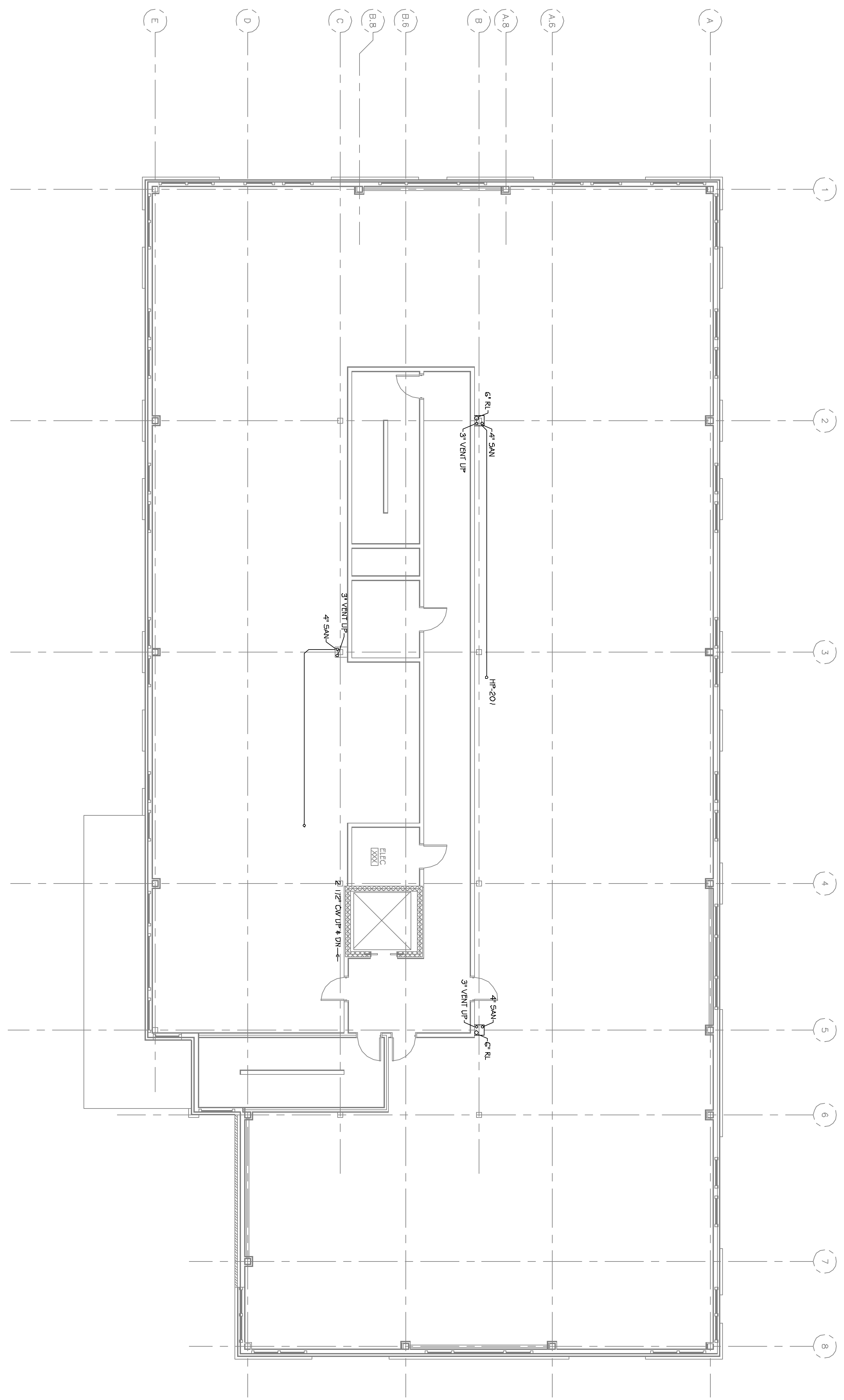
SECOND FLOOR PLAN SCALE 1/8"=1'-0"
