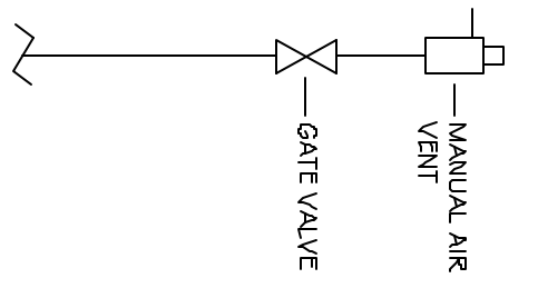
END OF MAIN AIR VENT DETAIL
