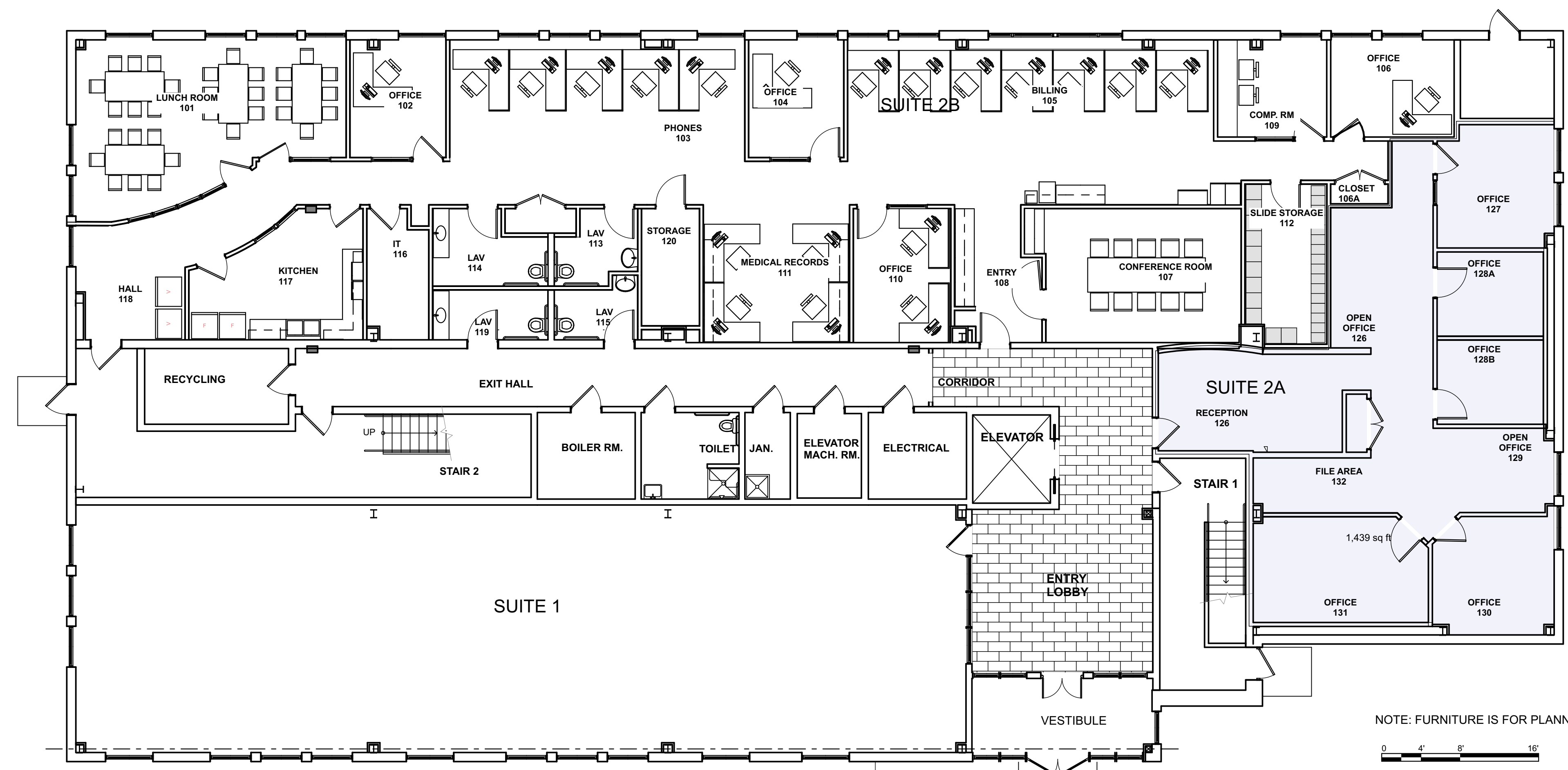
1 A1.8 1st FLOOR FURNITURE PLAN SCALE: 1/8" = 1'-0"
