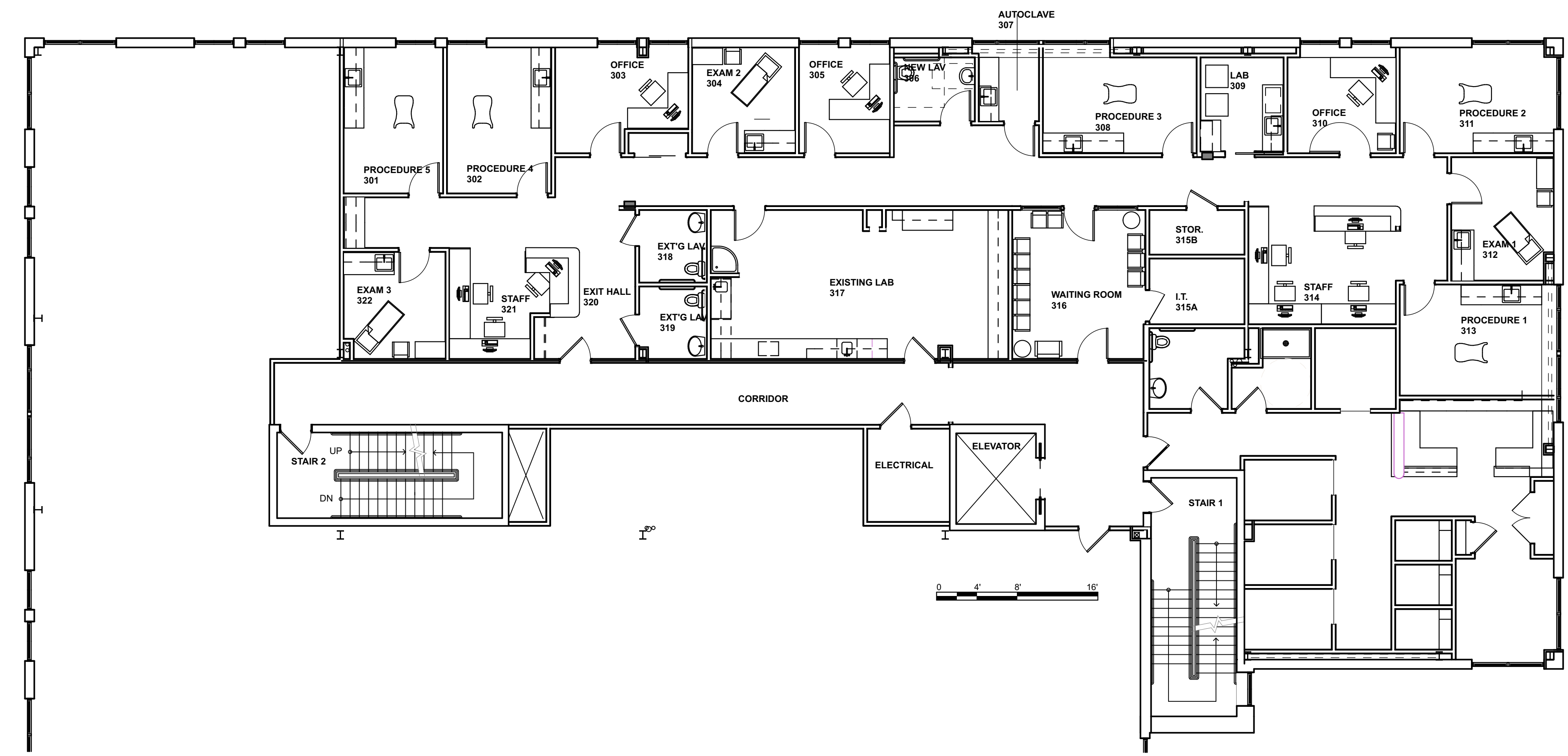
2 A1.8 3rd FLOOR FURNITURE PLAN SCALE: 1/8" = 1'-0"
