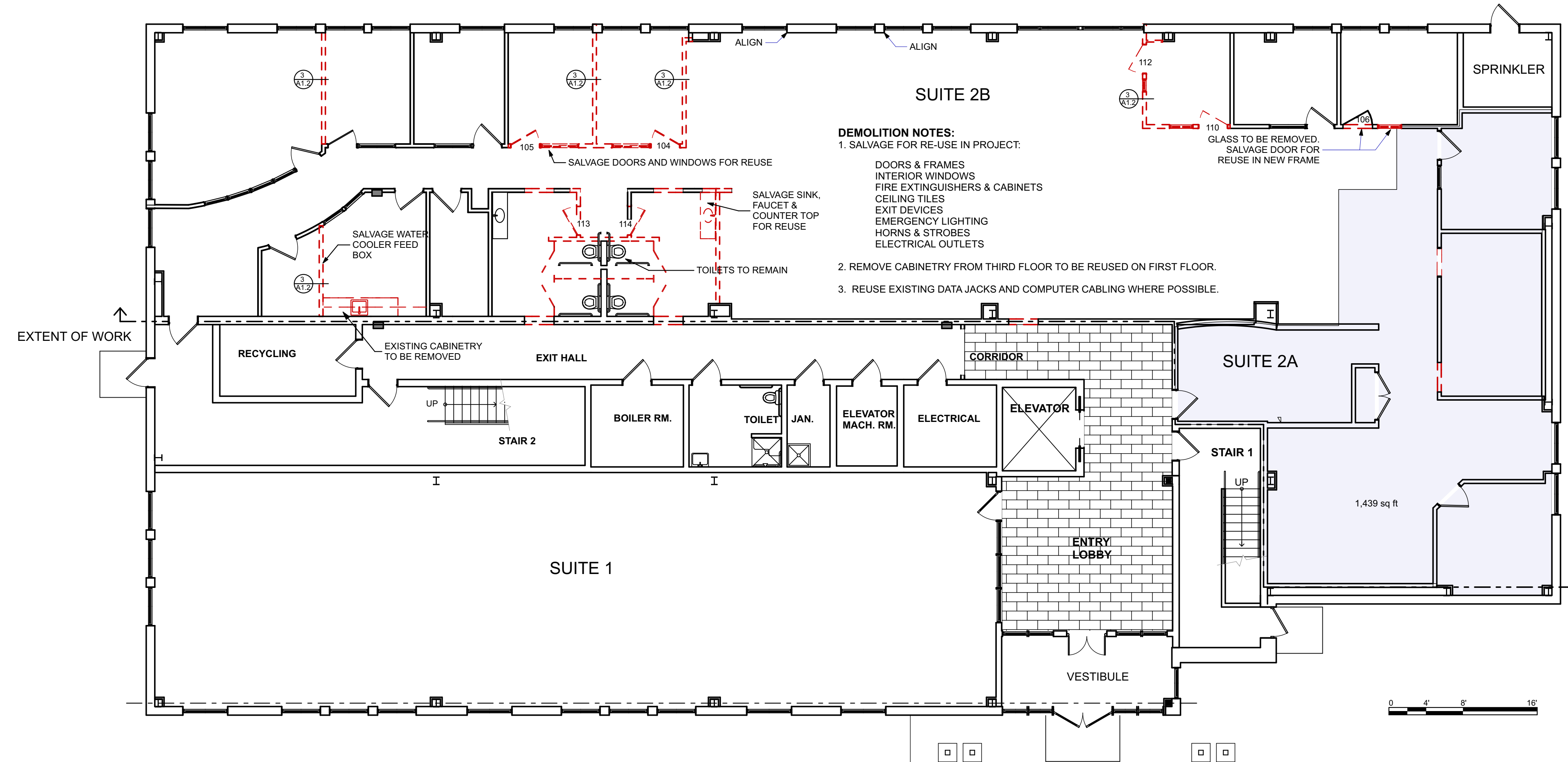
1 1st FLOOR DEMO PLAN SCALE: 1/8" = 1'-0"
