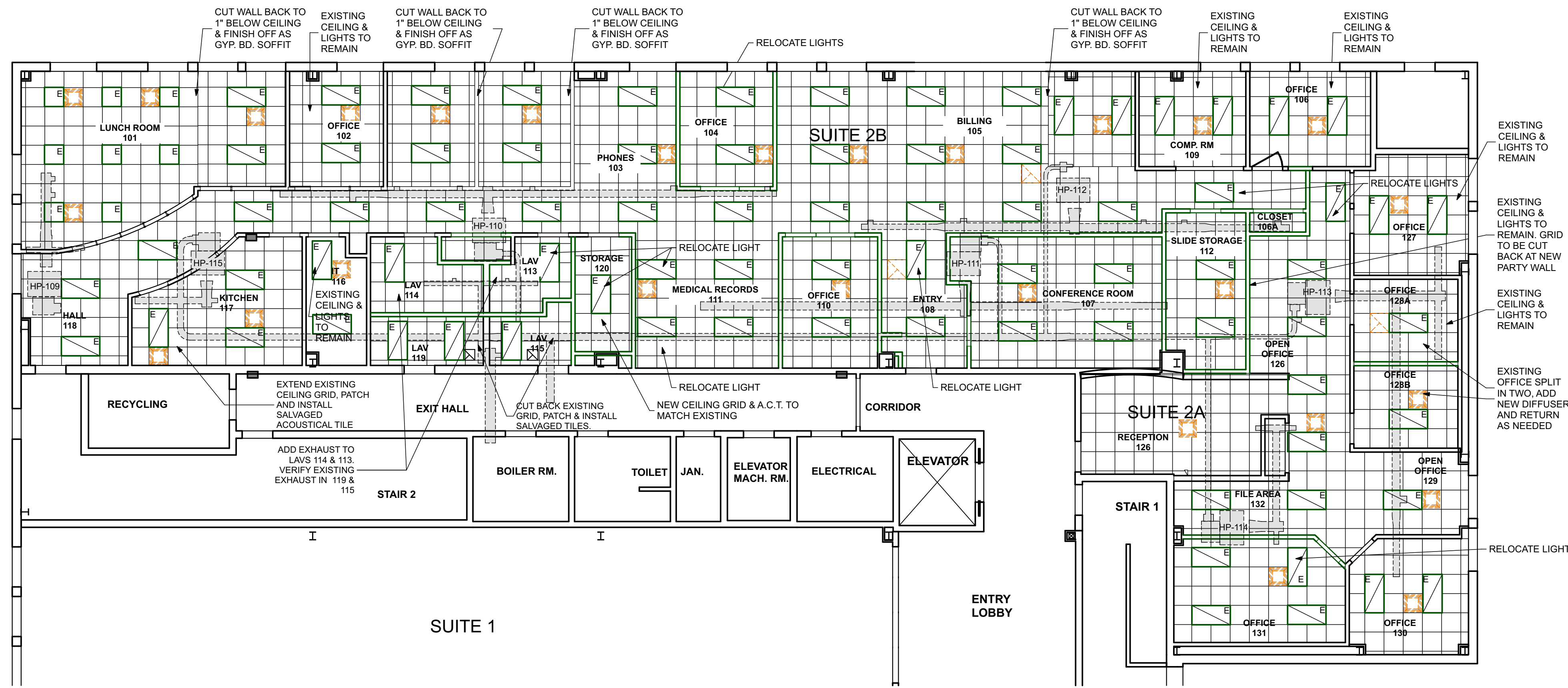
2 1st FLOOR REFLECTED CEILING PLAN SCALE: 1/8" = 1'-0"
