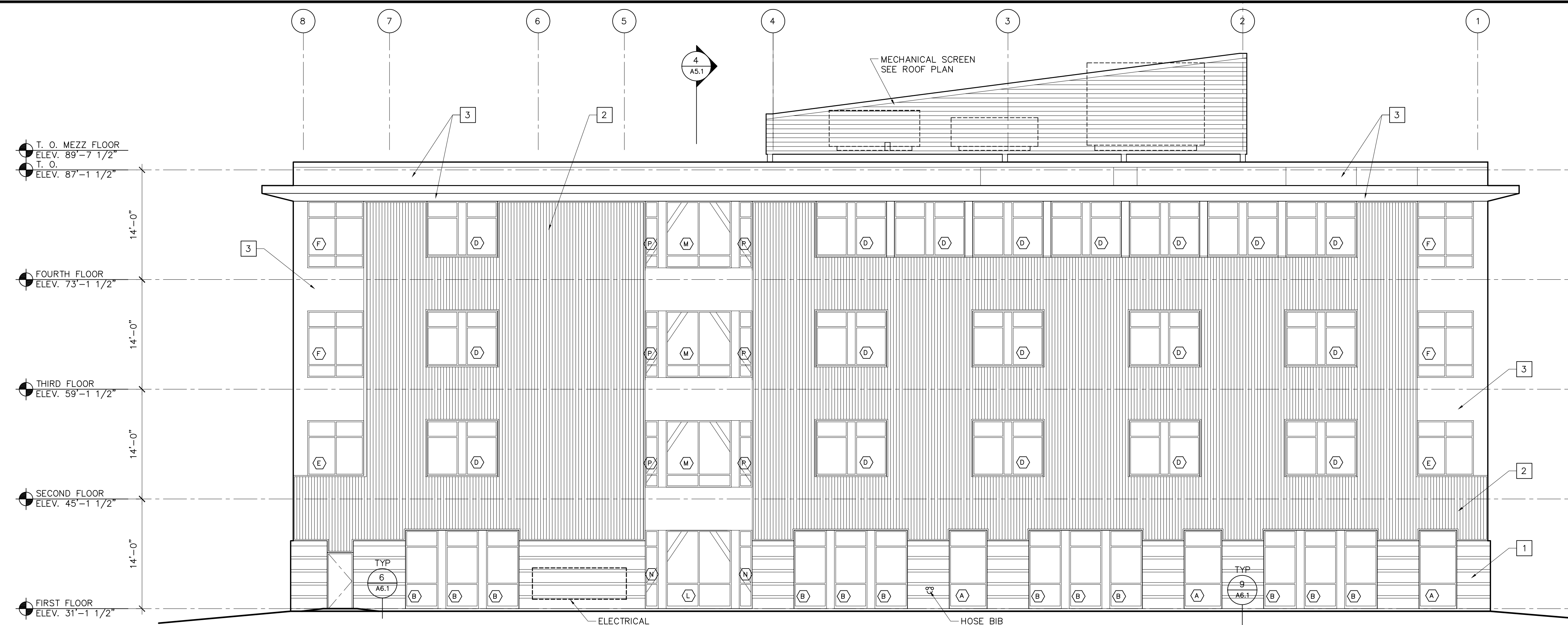
1 SOUTH ELEVATION 1/8" = 1'-0"
