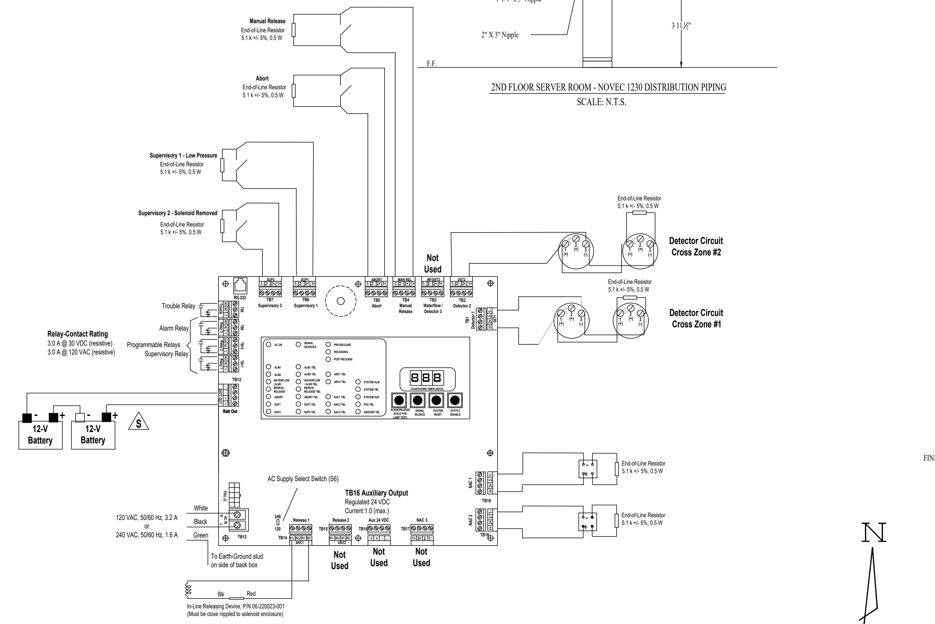
Kidde AEGIS Control Unit Installation Wiring Diagram Part No. 06-236730-001 Rev AA
