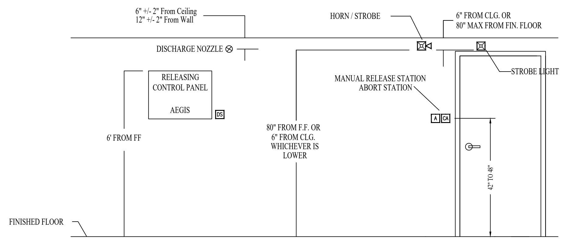
DEVICE ELEVATION DETAIL NOT TO SCALE
