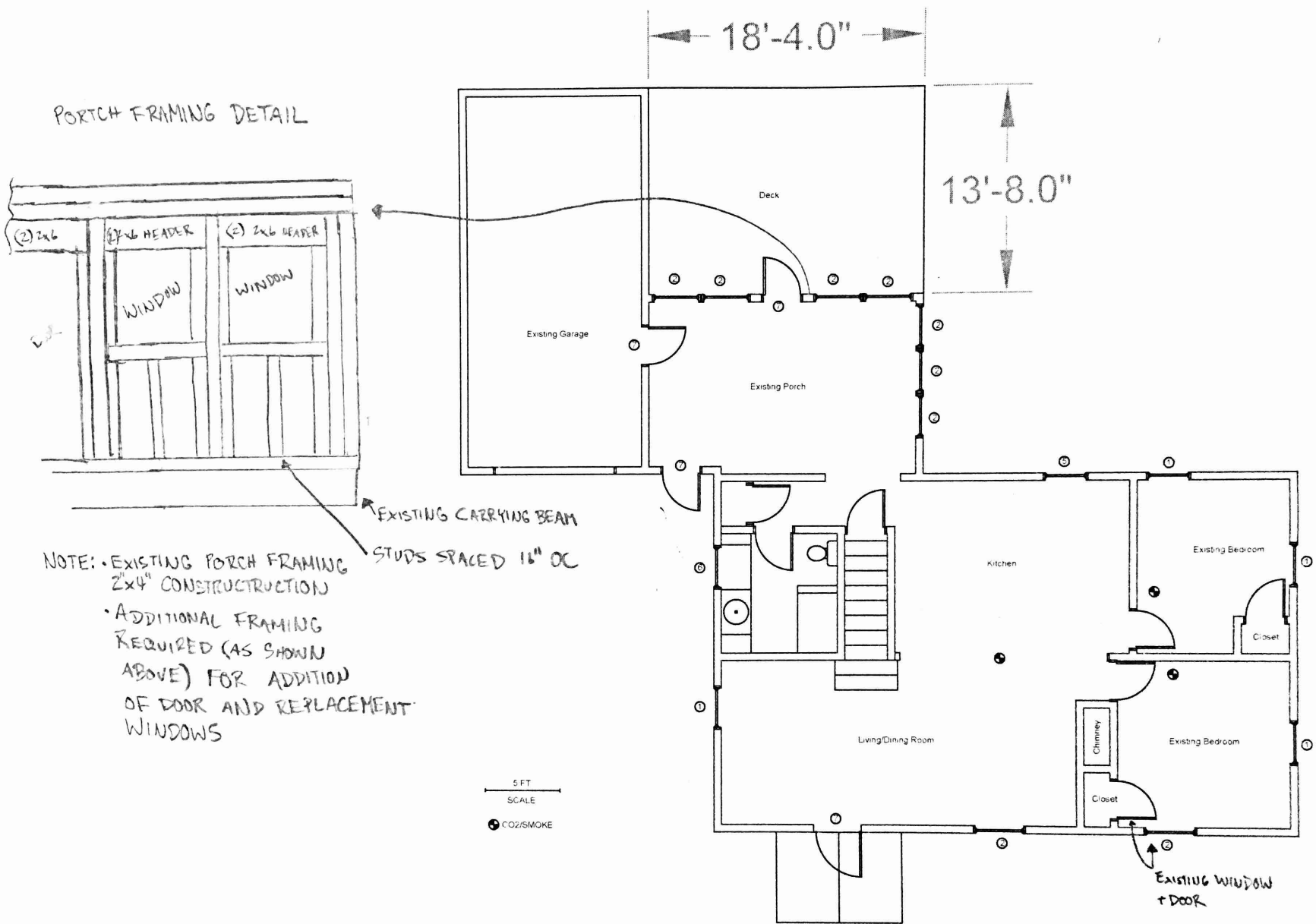
FIRST FLOOR PLAN VIEW (PROPOSED)
