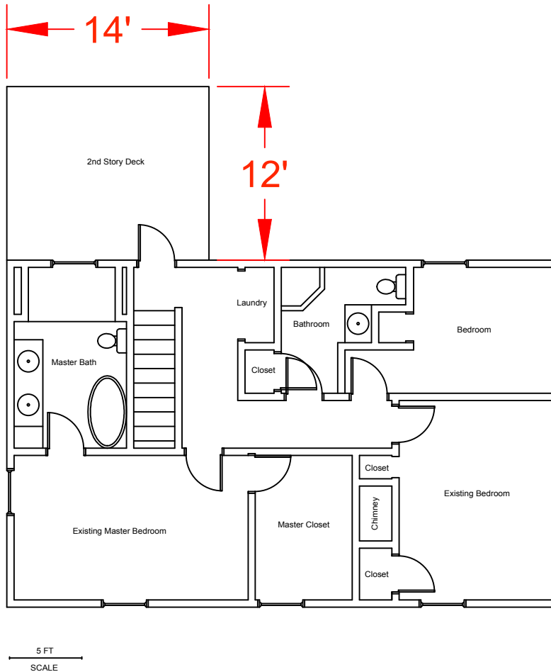
SECOND FLOOR PLAN VIEW (PROPOSED)
