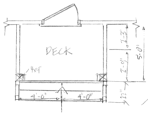
PORTICO PLAN SCALE 1/4" = 1'-0"
