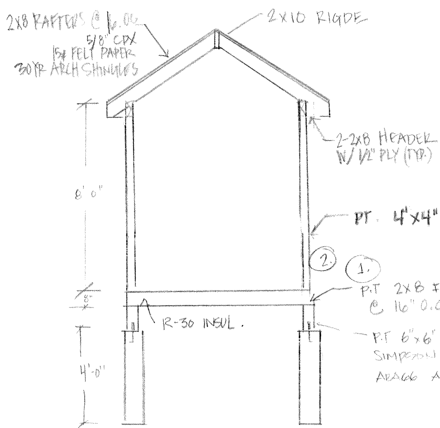
PORTICO CROSS-SECTION SCALE 1/4" = 1'-0"
