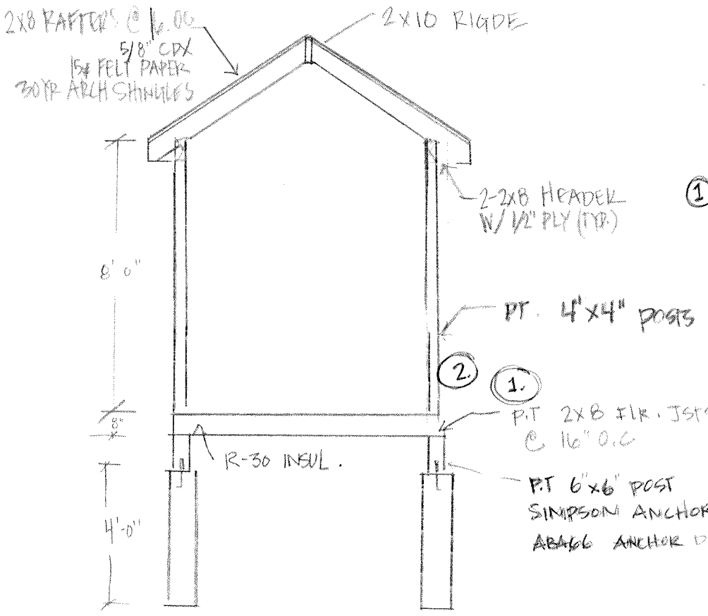
PORCH CROSS-SECTION SCALE 1/4" = 1'-0"
