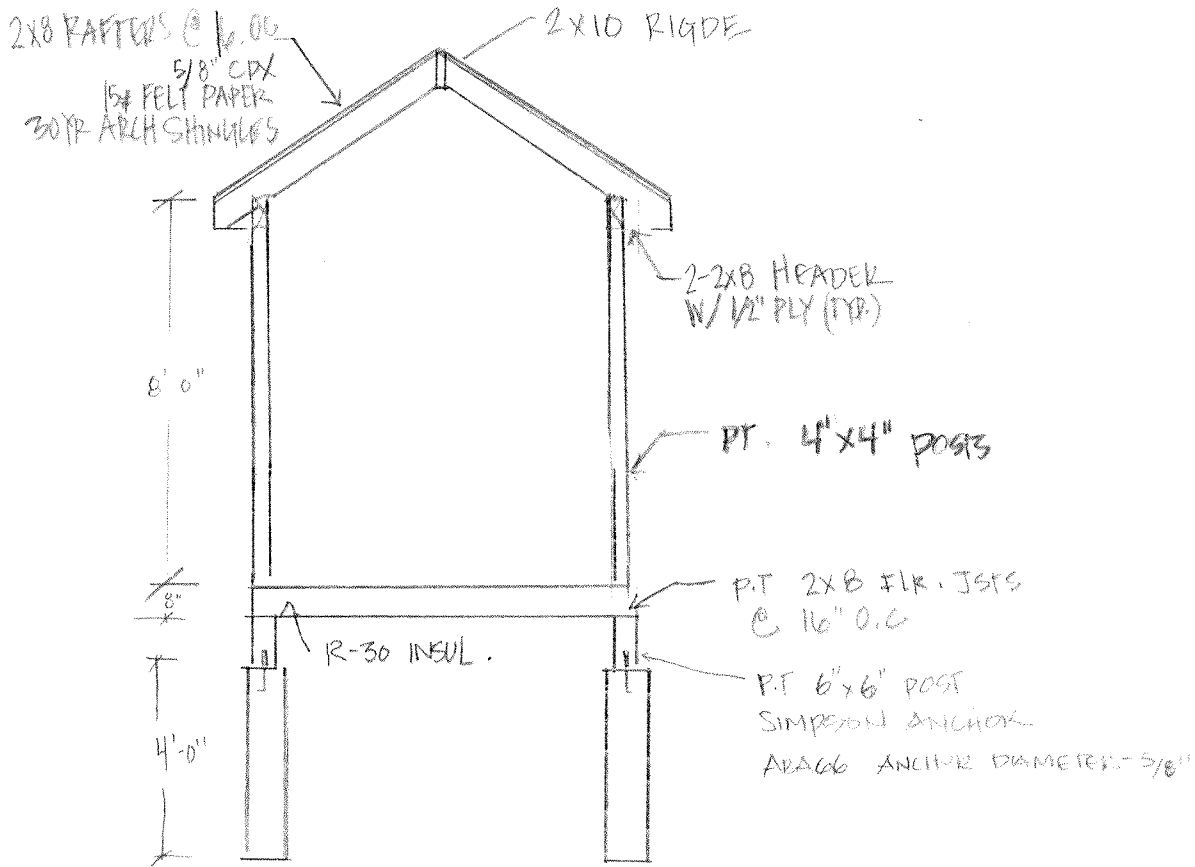
PORTICO CROSS-SECTION SCALE 1/4" = 1'-0"
