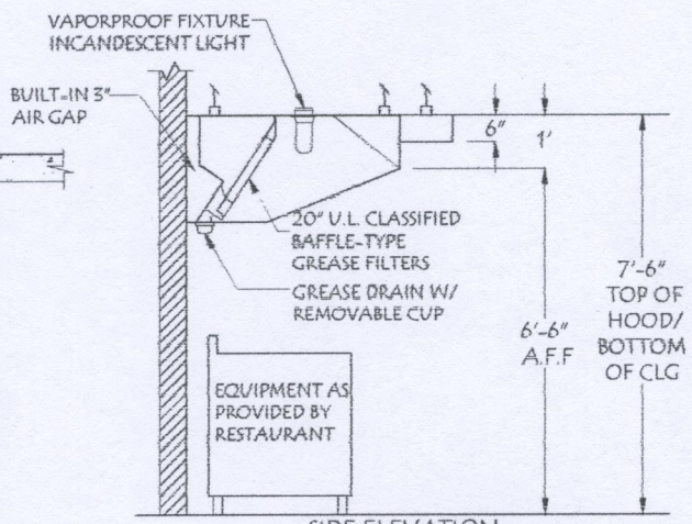
SIDE ELEVATION NOT TO SCALE
