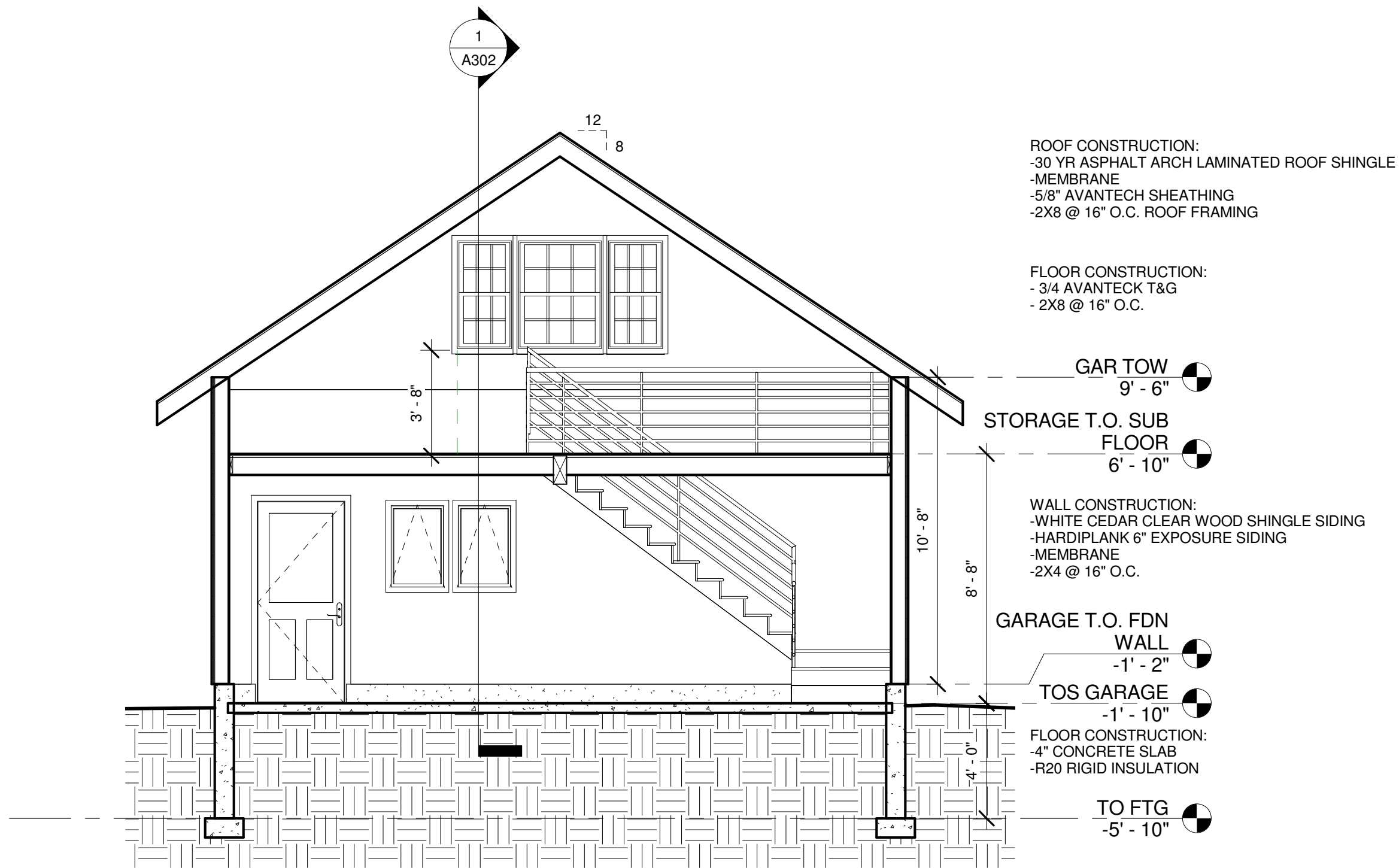
1 NORTH SOUTH GARAGE SECTION A301 1/4" = 1'-0"
