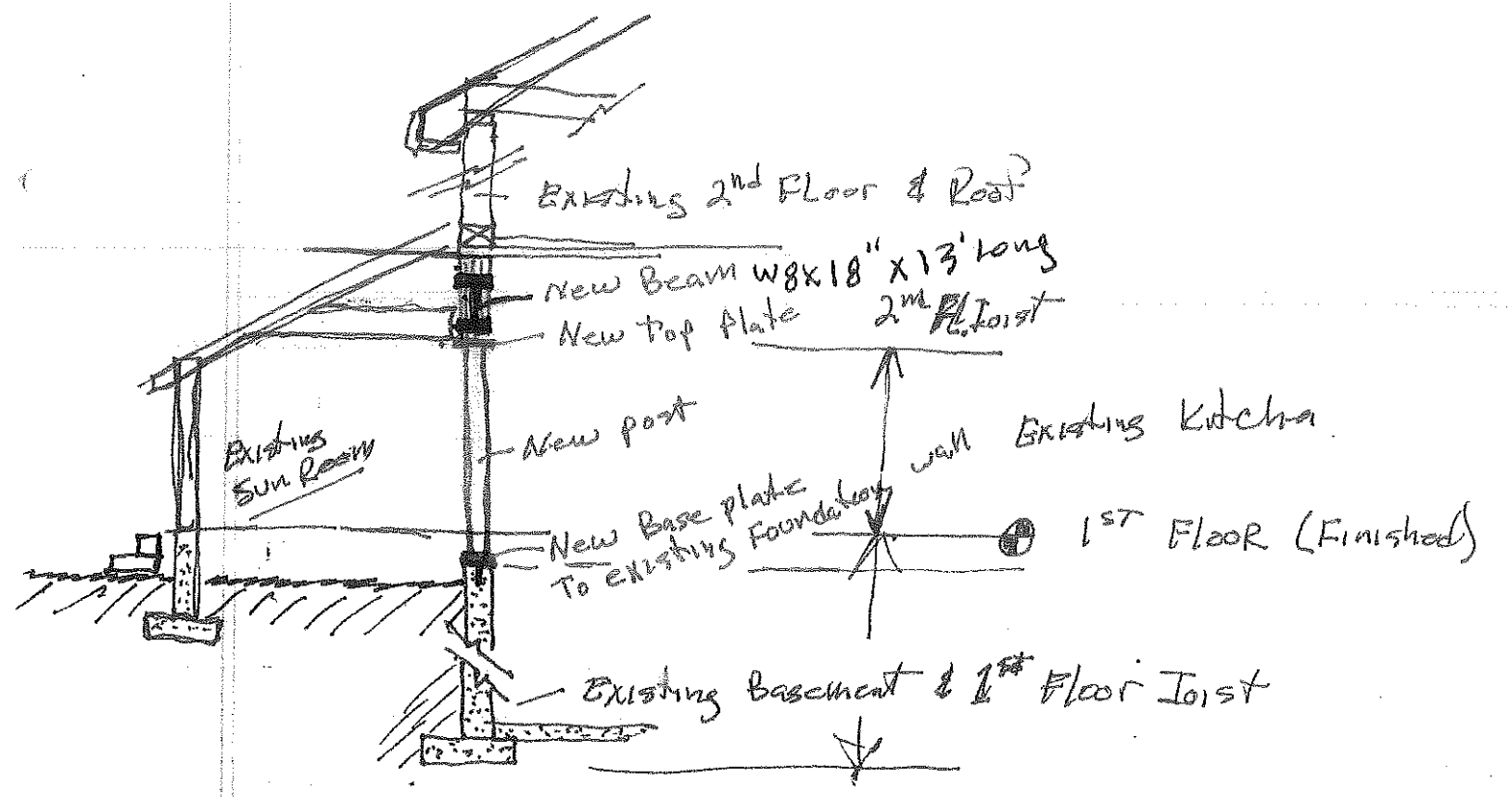
○ Sun Room & Kitchen Cross Section NTS
