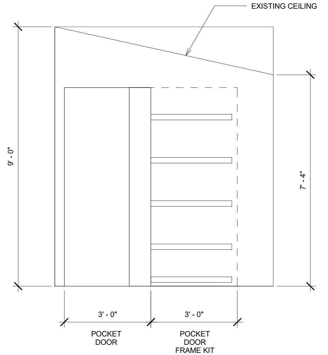
① New Wall Detail 1/2" = 1'-0"
