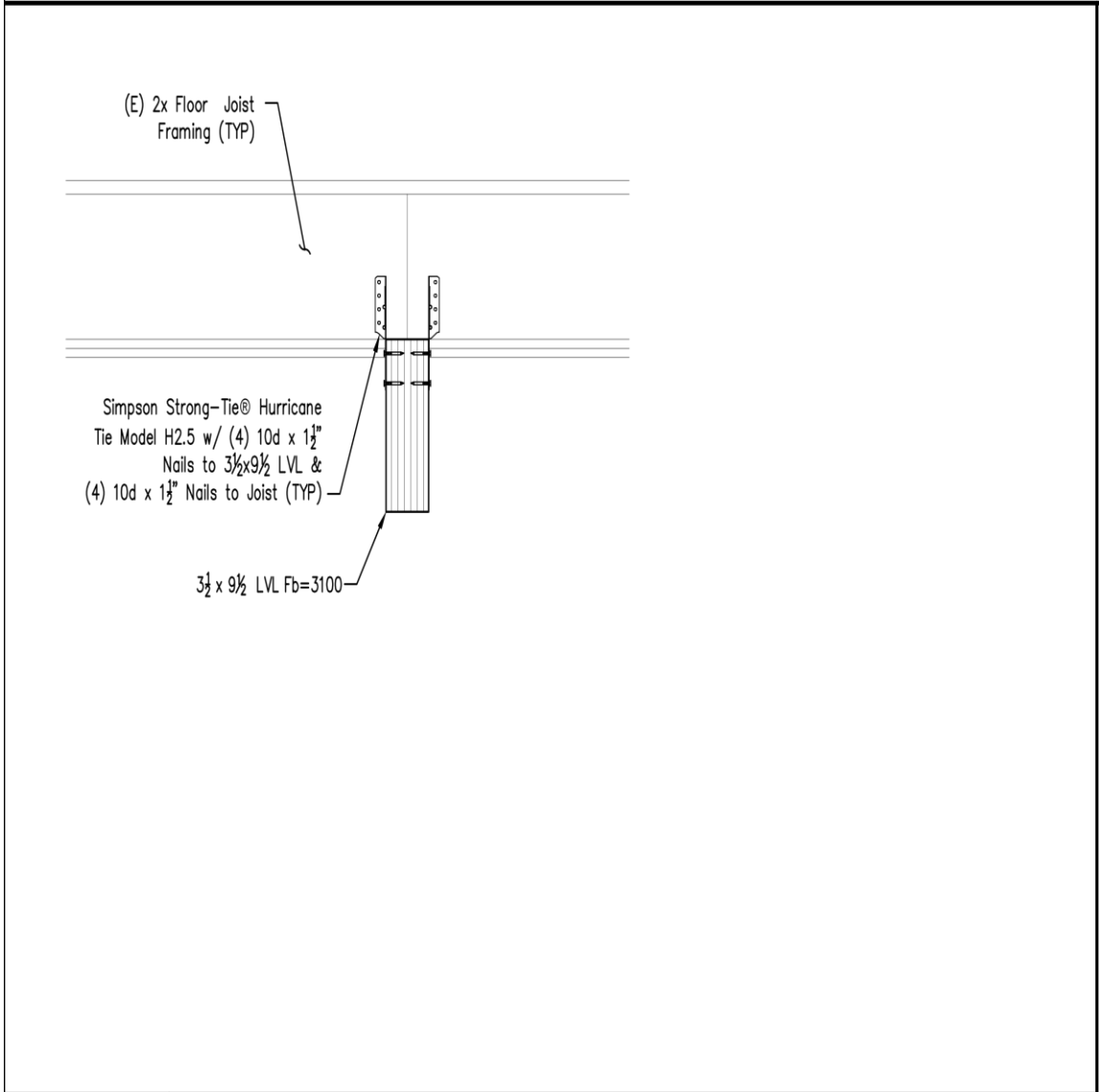
S2 FLOOR FRAMING CONNECTION DETAIL 1-1/2" = 1'-0"
