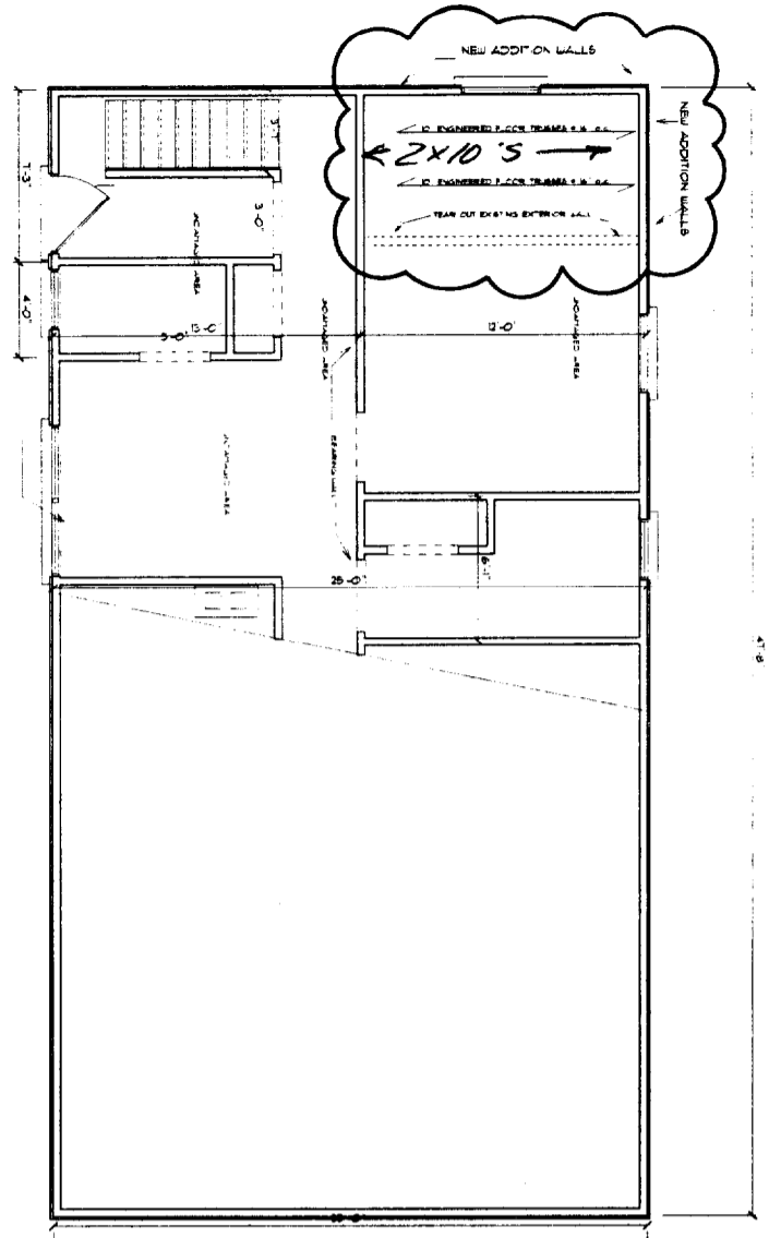
1ST FLOOR LAYOUT SCALE 1/4" = 1'-0"
