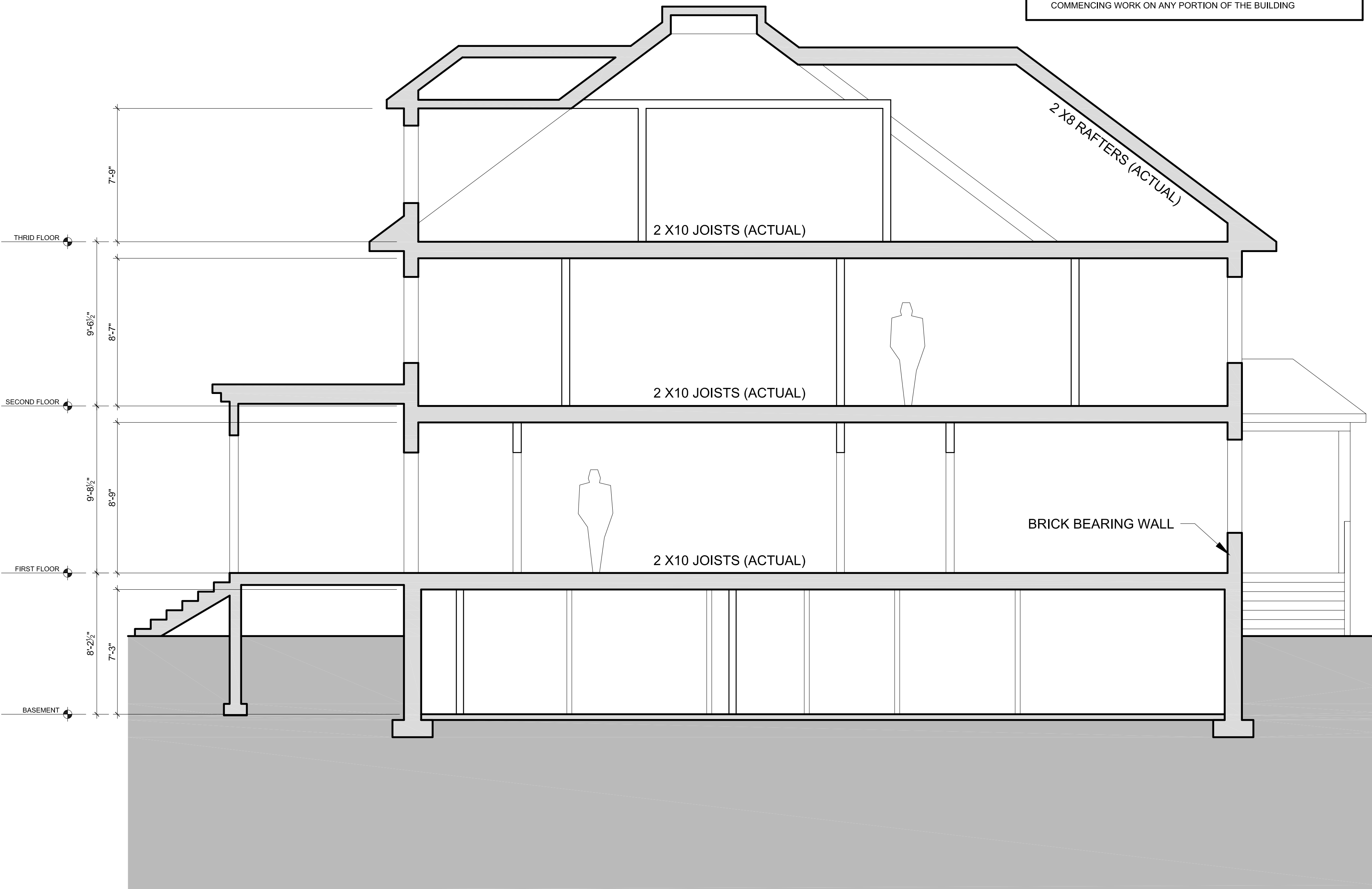
1 EXISTING CONDITIONS BUILDING SECTION EX3.1 1/4" = 1'-0"
