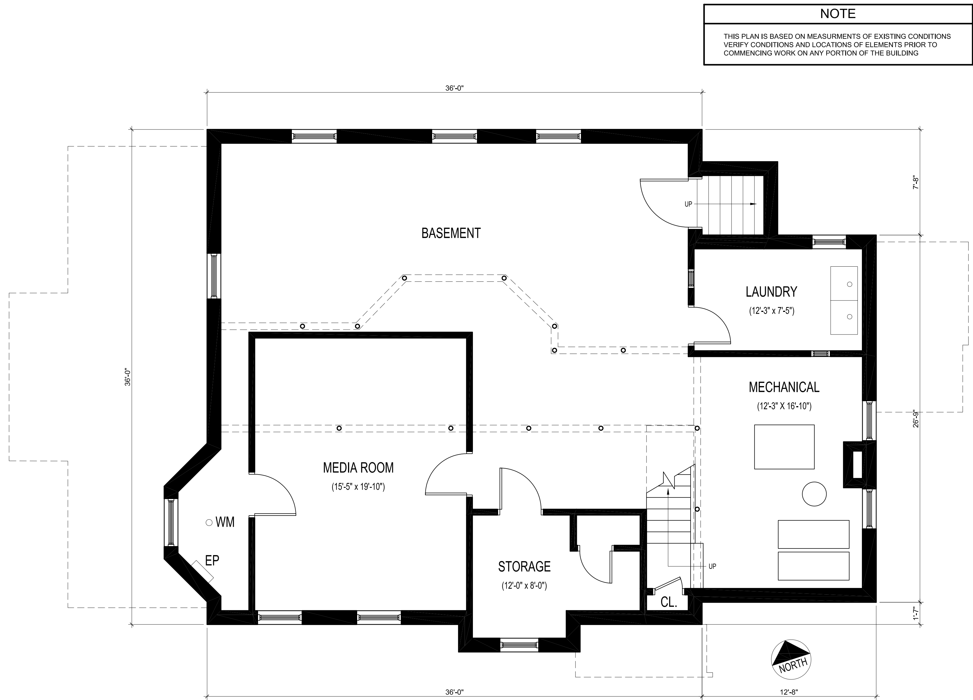
1 EXISTING BASEMENT PLAN EX1.0 1/4" = 1'-0"
