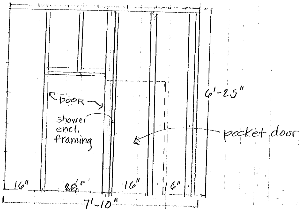
NW Elevation
