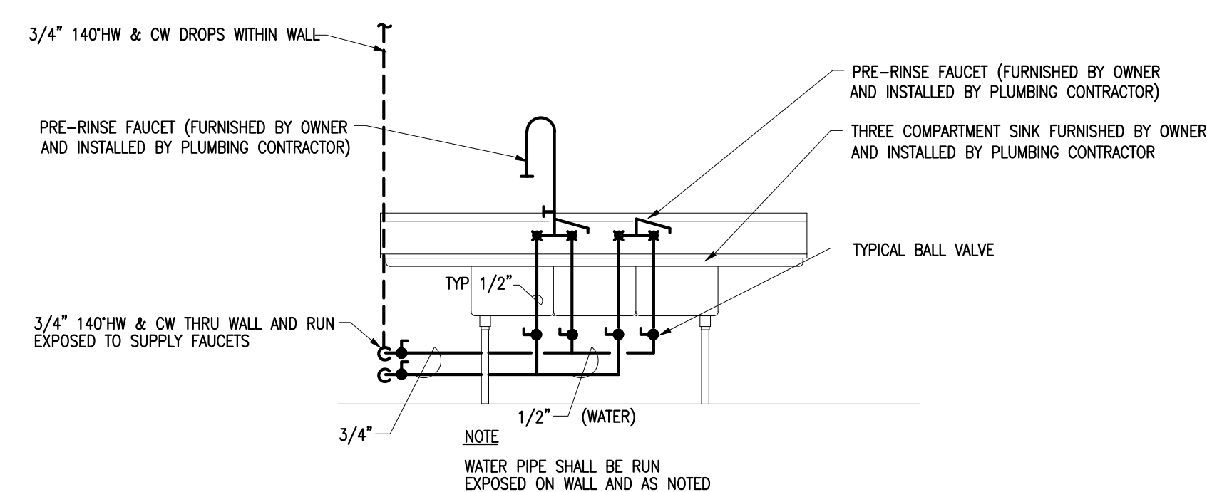
5 TRIPLE COMPARTMENT POT SINK NOT TO SCALE
