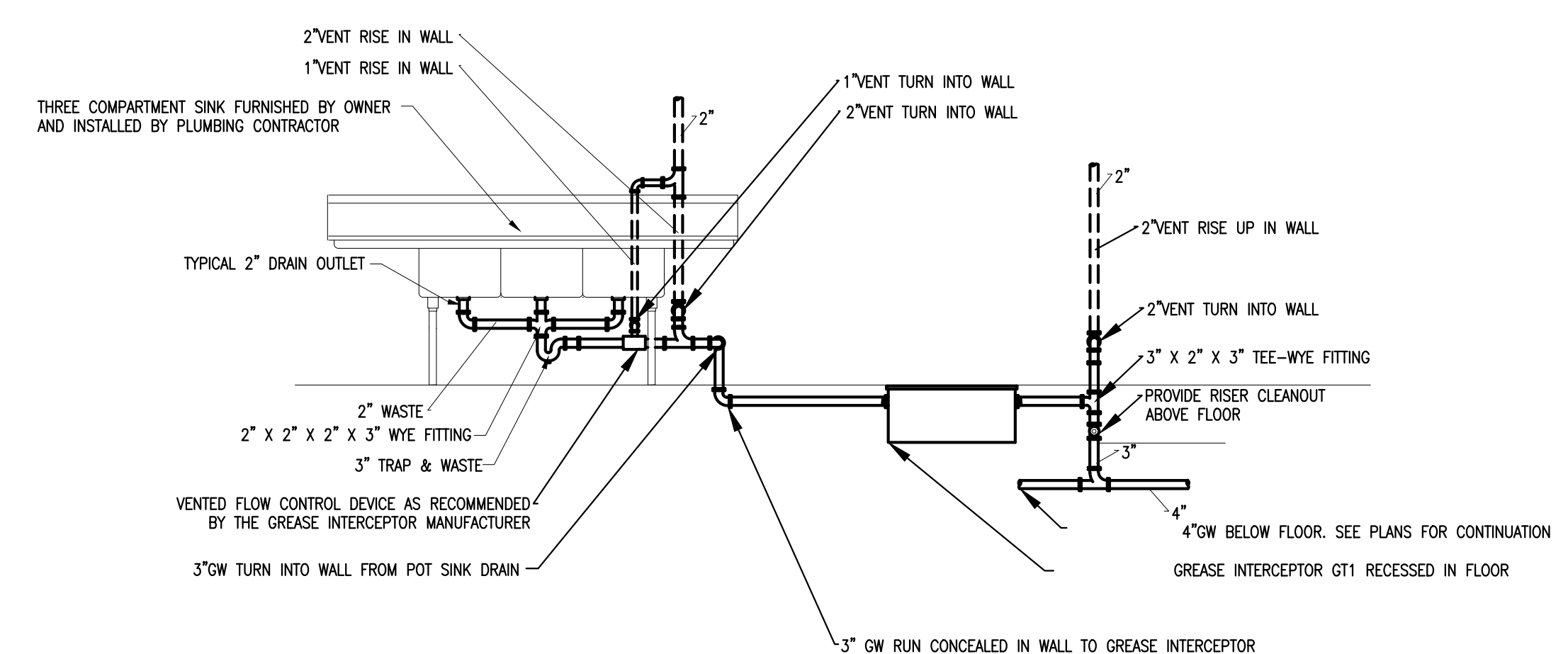
4 TRIPLE COMPARTMENT POT SINK NOT TO SCALE
