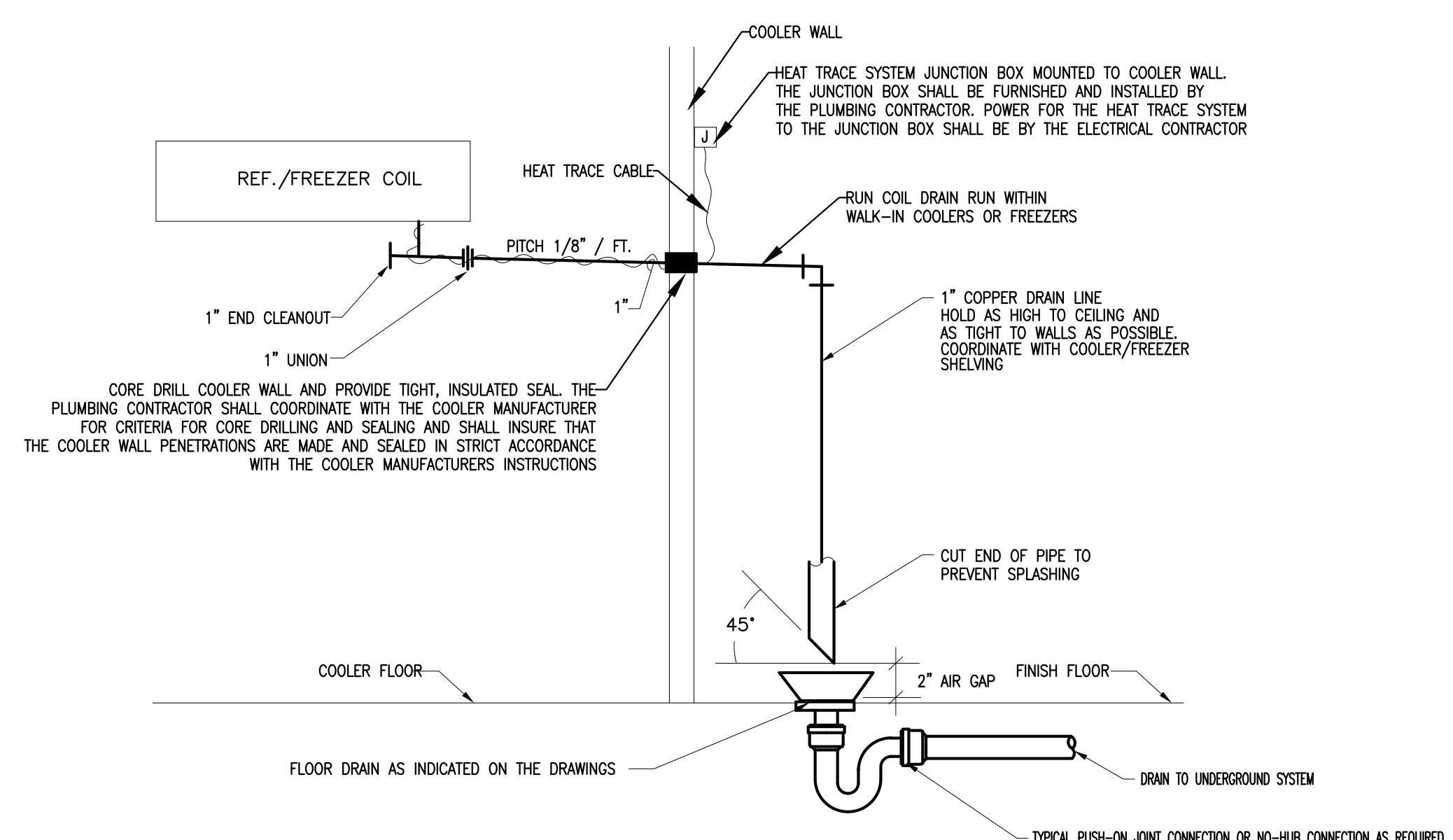
2 TYPICAL COOLER/FREEZER COIL DRAIN NOT TO SCALE
