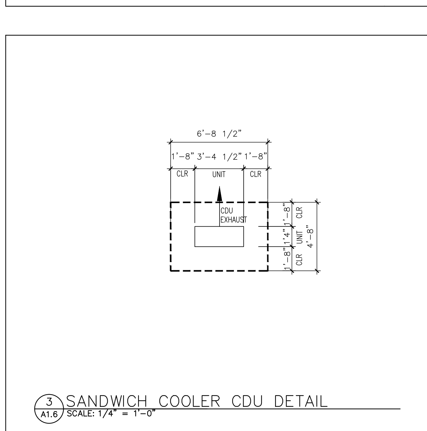
3 SANDWICH COOLER CDU DETAIL A1.6 SCALE: 1/4" = 1'-0"
