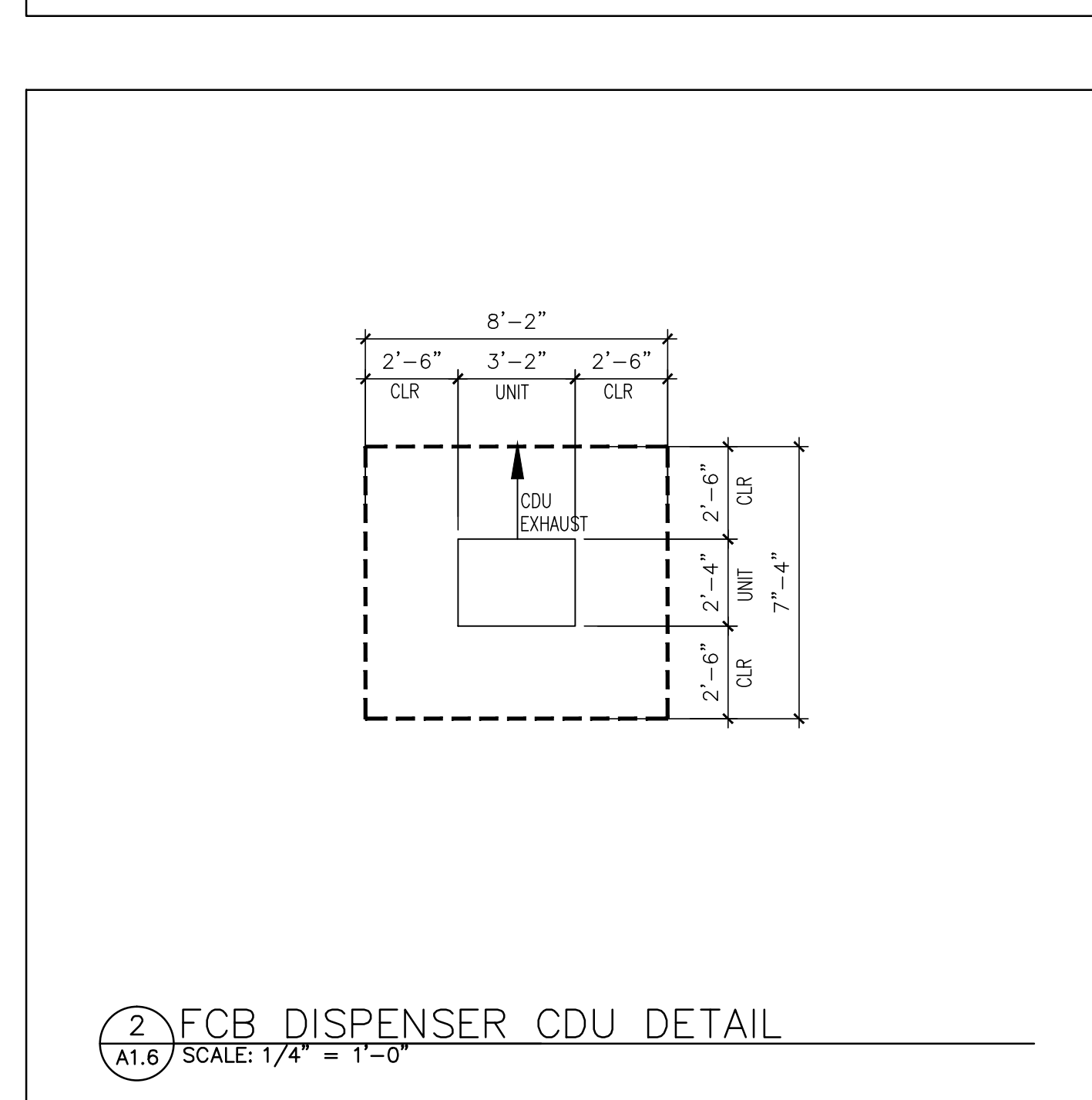
2 FCB DISPENSER CDU DETAIL A1.6 SCALE: 1/4" = 1'-0"
