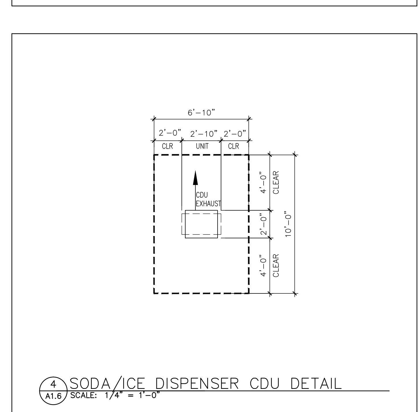
4 SODA/ICE DISPENSER CDU DETAIL A1.6 SCALE: 1/4" = 1'-0"
