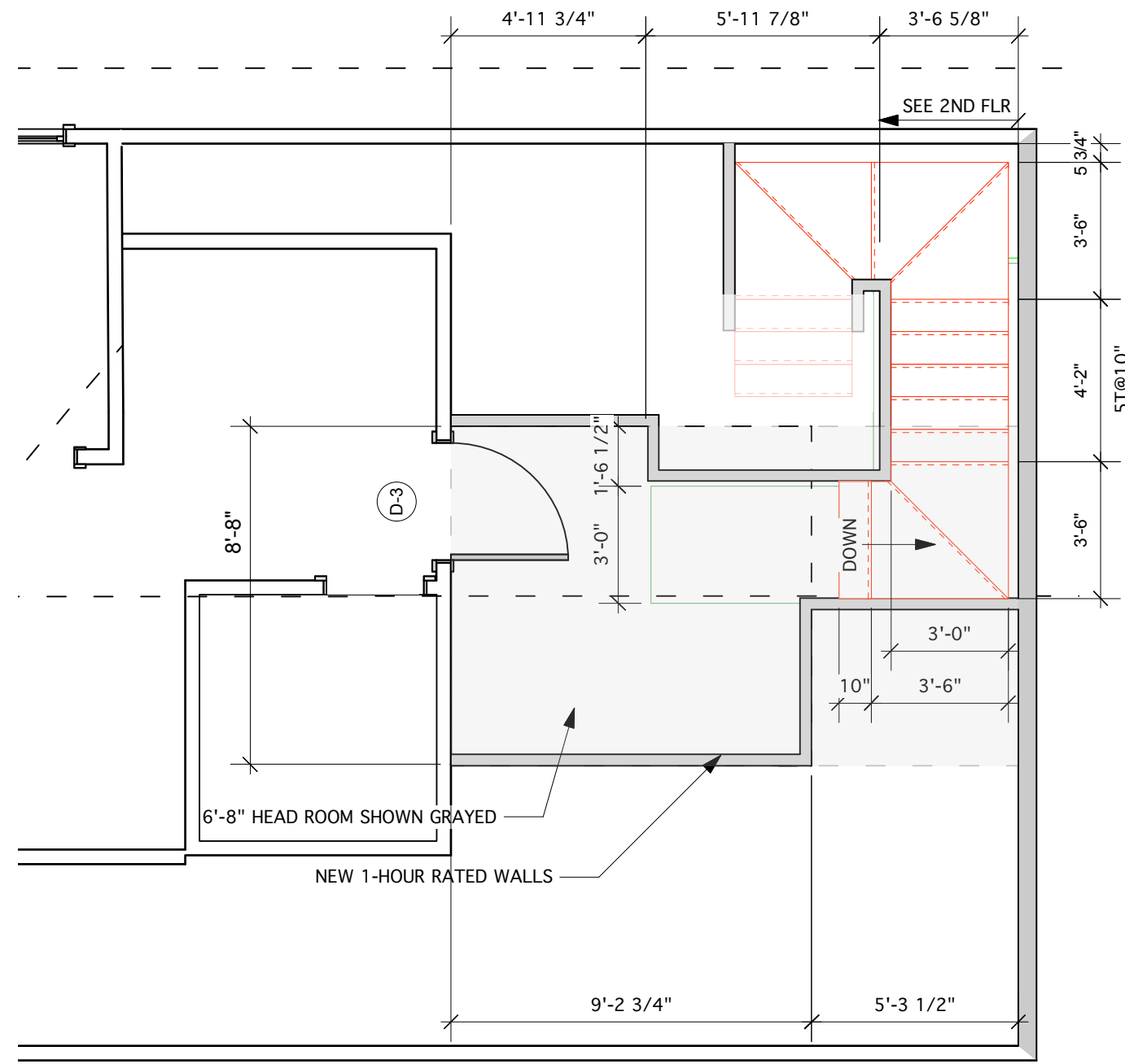
3 THIRD FLOOR PLAN Scale: 1/4" = 1'-0"
