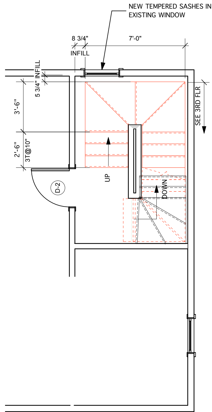
2 SECOND FLOOR PLAN Scale: 1/4" = 1'-0"
