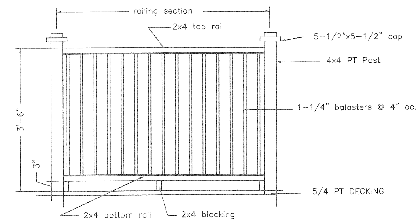
SECTION D Typical Railing Detail Scale: 3/4" = 1'-0"
