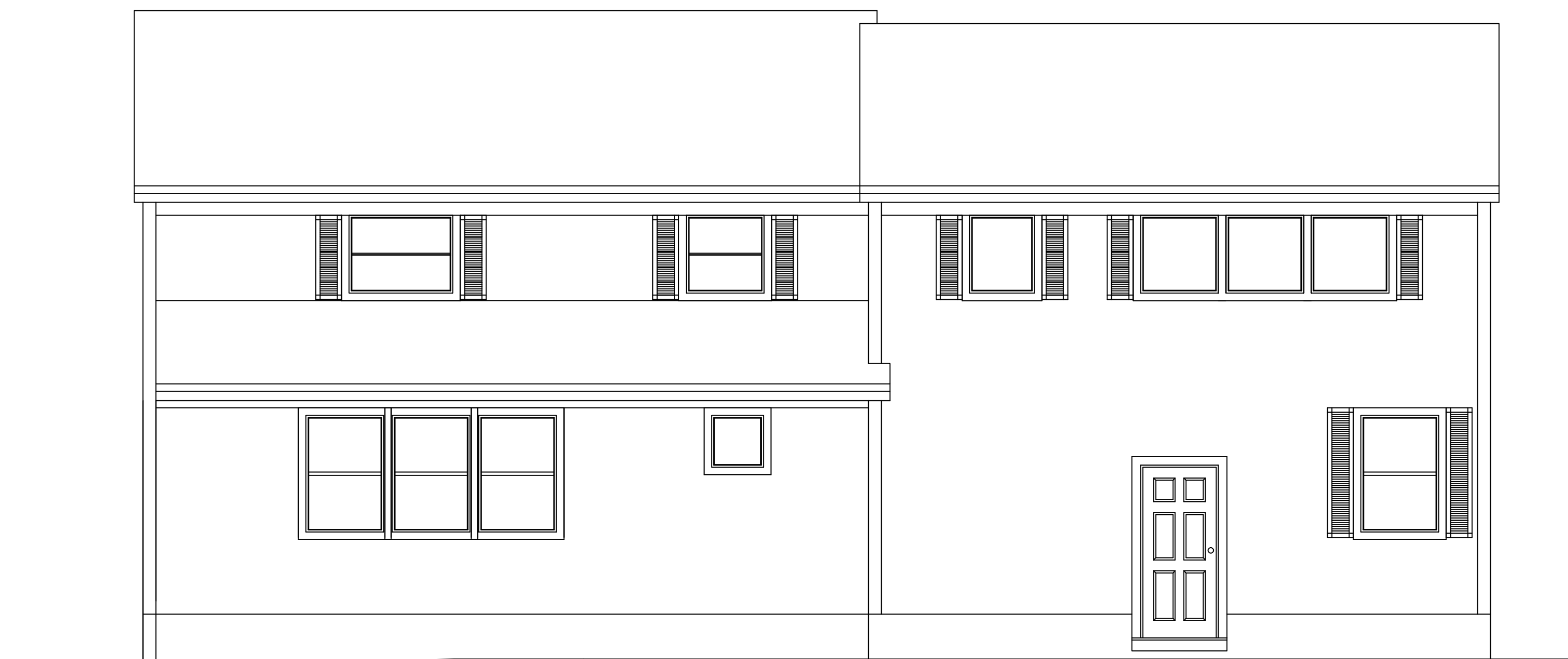
NEW REAR ELEVATION
