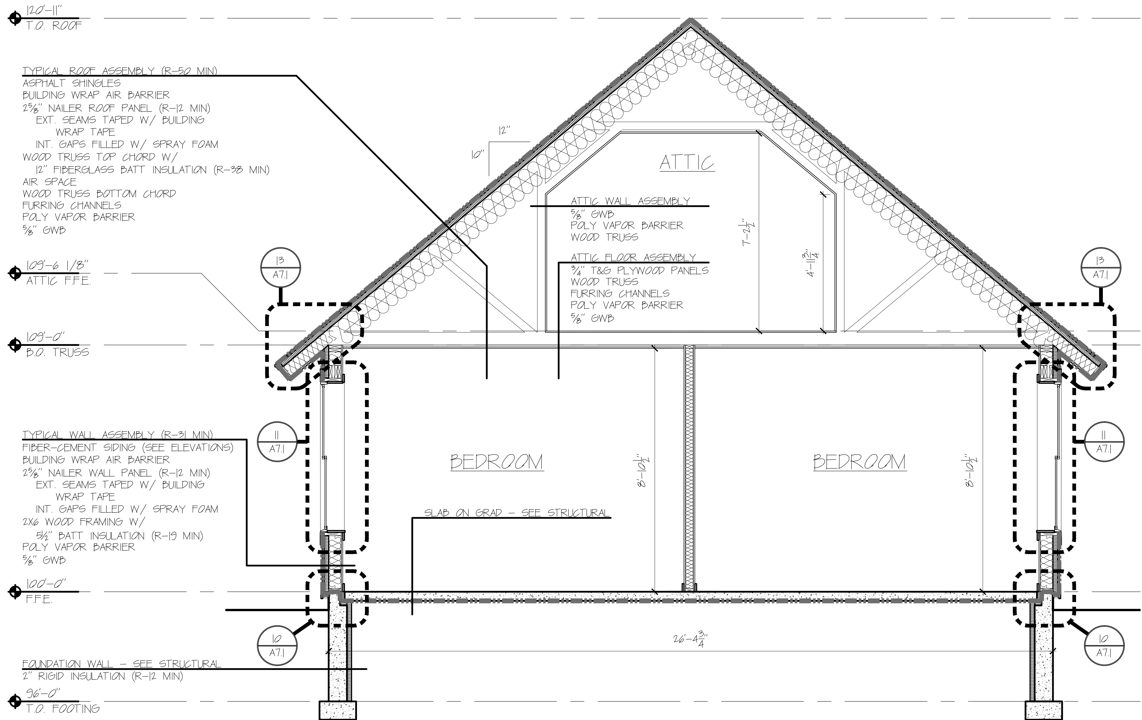
10 BEDROOM BUILDING SECTION 0 2'-0" SCALE: 1/2" = 1'-0"
