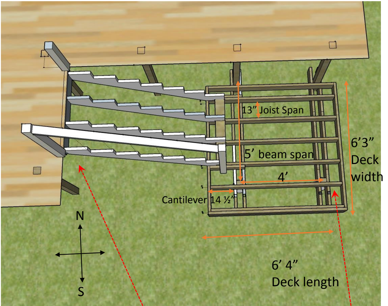
Stringer connector to existing deck Rim Joist
