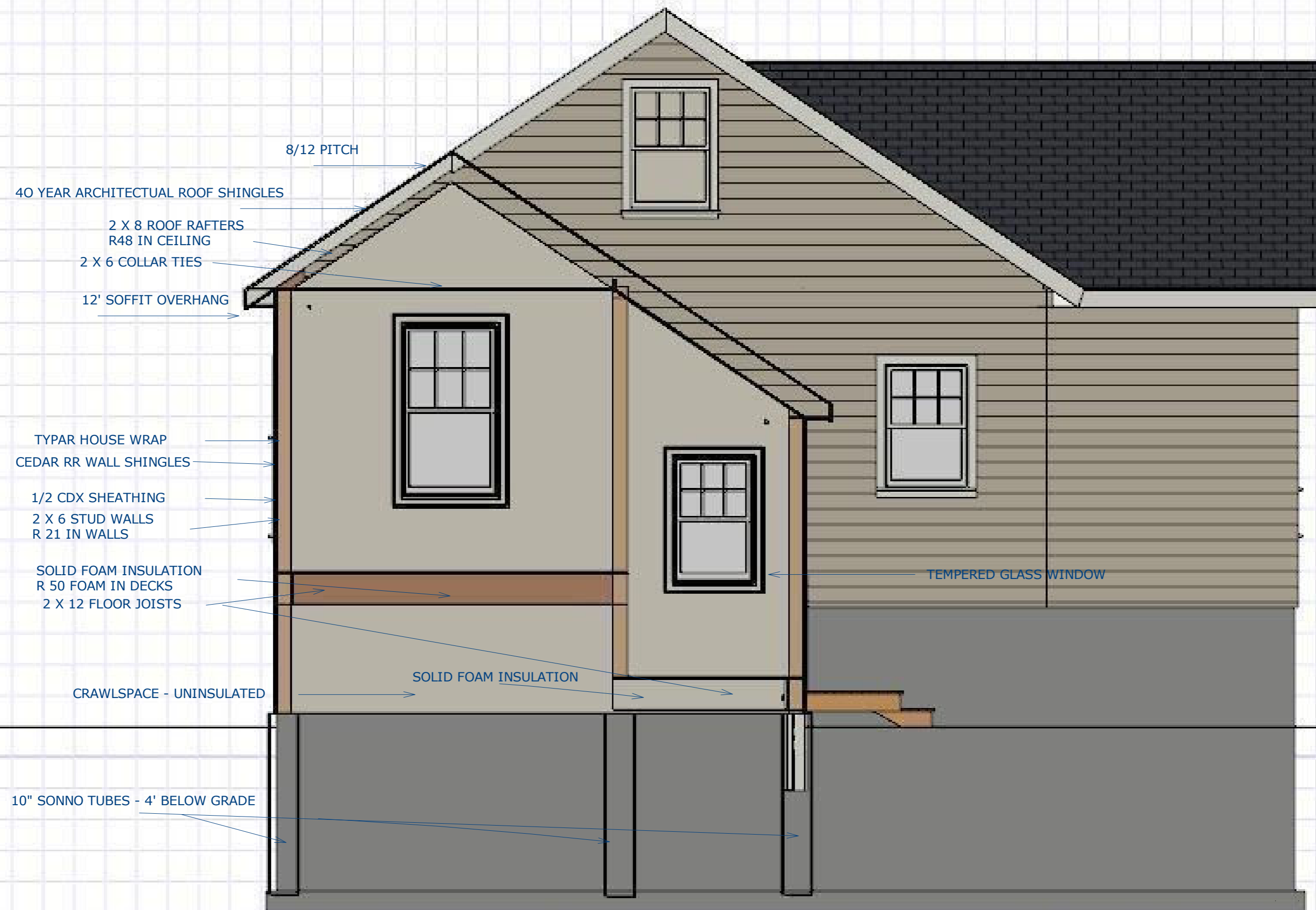
NORTH ELEVATION
