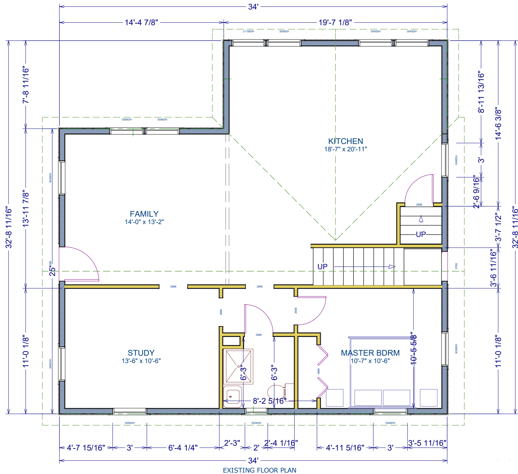
EXISTING FLOOR PLAN
