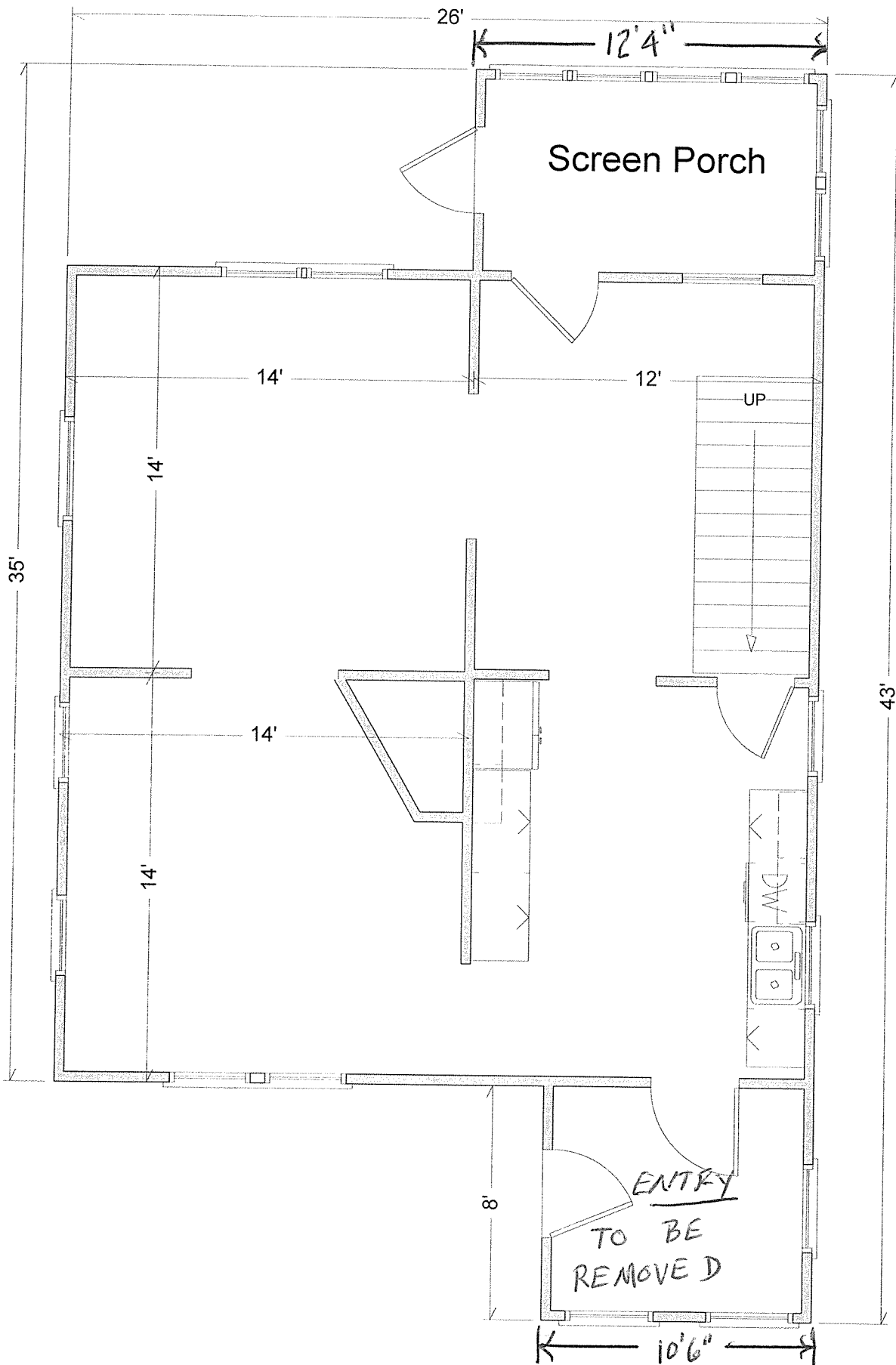
EXISTING CONDITION FIRST FLOOR
