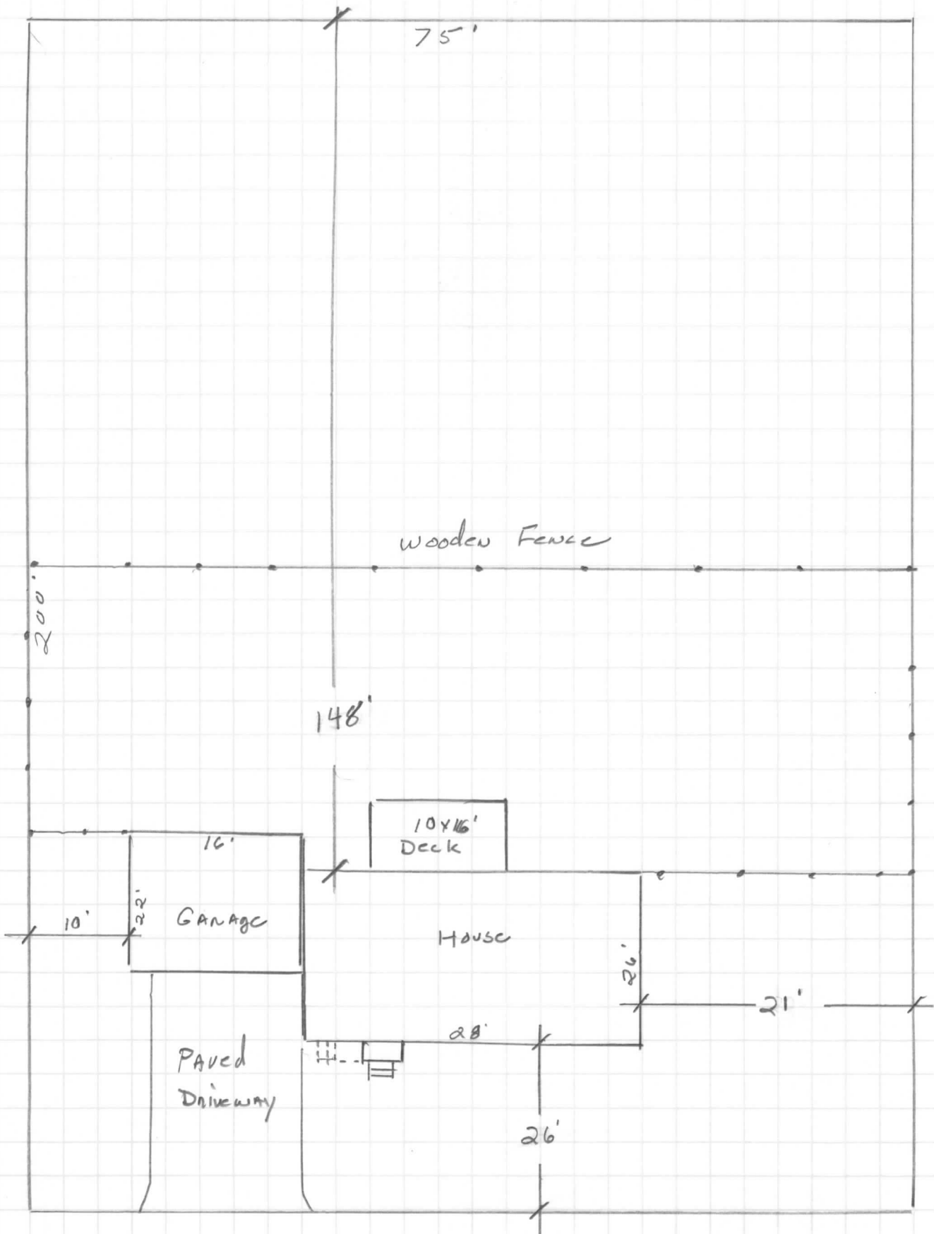
A4 Plot Plan
