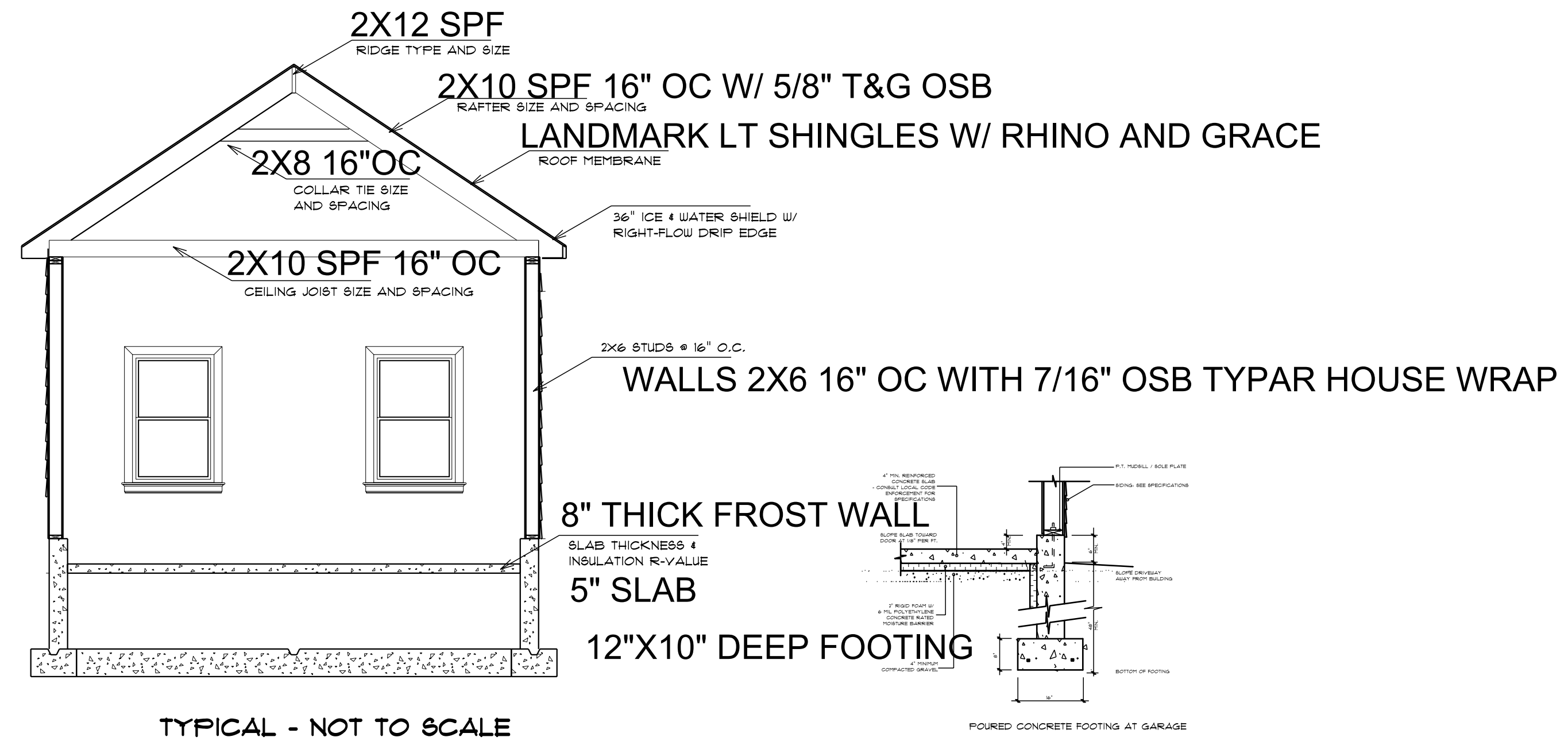
SECTION B SCALE: 1/4" = 1'-0" TYPICAL - NOT TO SCALE *HOMEOWNER/CONTRACTOR TO SPECIFY VALUES FOR EACH OF THE CALLOUTS. SOME CALLOUTS MAY NOT BE APPLICABLE*
