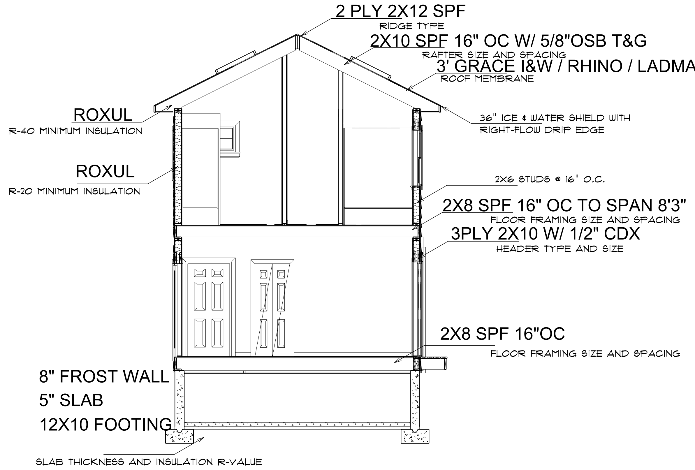
SECTION A SCALE: 1/4" = 1'-0" TYPICAL - NOT TO SCALE *HOMEOWNER/CONTRACTOR TO SPECIFY VALUES FOR EACH OF THE CALLOUTS. SOME CALLOUTS MAY NOT BE APPLICABLE*
