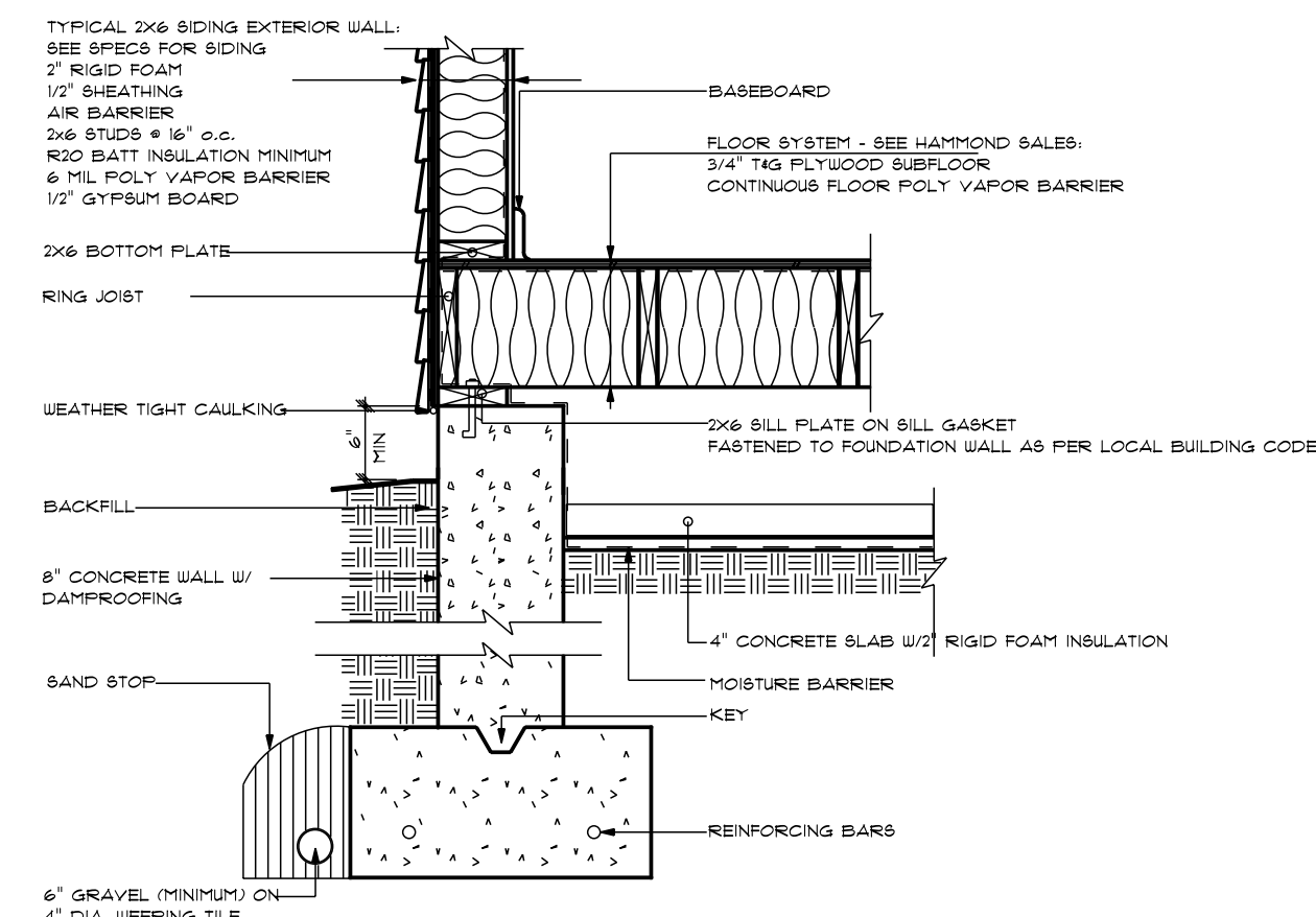
2X6 MUDROOM TYPICAL
