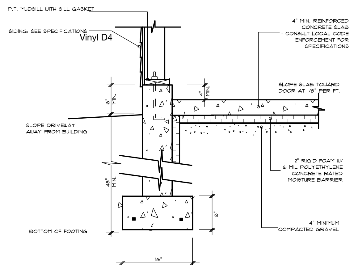
POURED CONCRETE FOOTING AT GARAGE
