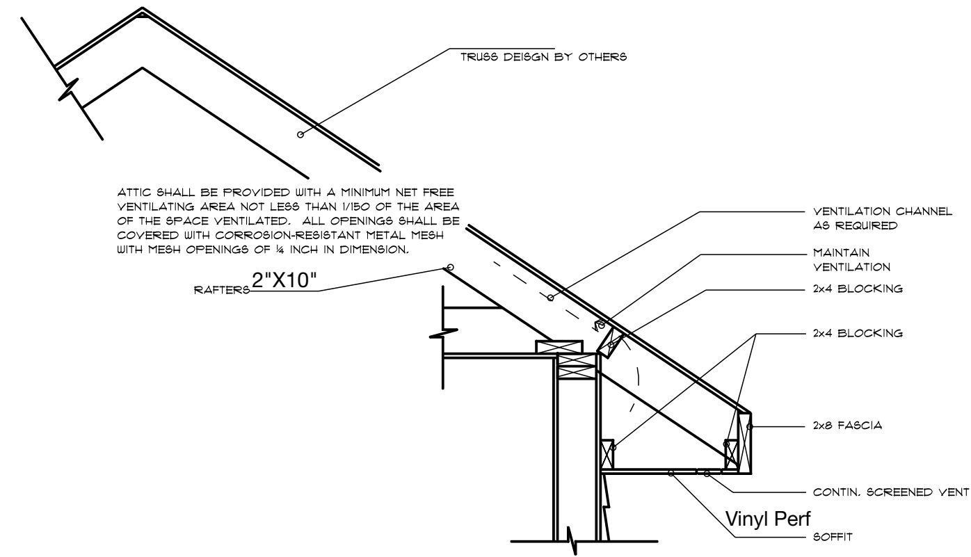
ROOF VENTILATION SOFFITED EAVE SIDING
